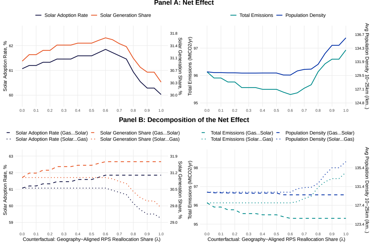
Figure 9. Counterfactual Analysis: Geography-Aligned RPS Reallocation. This figure traces the path from the observed RPS allocation ( \lambda = 0 ) to the proportional geography-aligned allocation ( \lambda = 1 ). \lambda fixes a fraction of that total reallocation, sequenced to maximize solar creation where renewable policy tightens and to minimize solar loss where it relaxes. Panel A reports the net effect: the left plot shows the solar adoption rate (left axis) and the solar generation share (right axis); the right plot shows total emissions (left axis, applying 0.37 tCO 2 per gas MWh) and the average population density in the 10–25 km ring around project sites (right axis). Panel B decomposes each net path into the gas-to-solar switches (dashed) and the solar-to-gas switches (dotted). Total installed capacity is fixed along the reallocation path.
