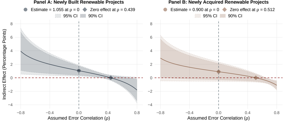
Figure 3. Sensitivity of Renewable Transition Mechanisms to Omitted Variable Bias. This figure shows how the indirect point estimates in Table 4 change with the assumed correlation \rho between mediator-equation and outcome-equation errors ( \rho = \text{Corr}(\varepsilon^M, \varepsilon^Y) ), following Imai et al. (2010). Panel A uses owned capacity in newly built renewable projects; Panel B uses owned capacity acquired from existing renewable projects. Both measures are benchmarked against total owned capacity fixed at regulatory event year -1 . Within each panel, the circle identifies the estimate at \rho = 0 , and the diamond identifies the correlation that reduces it to zero. The horizontal dashed line marks zero indirect effect, and the vertical dashed line marks \rho = 0 . The lighter outer region and darker inner region show 95% and 90% pointwise confidence intervals, respectively.
