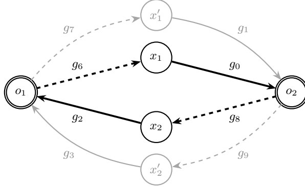
Fig. 1. The arrows of the draft state of Section 7. Double circles are the free agents. Dashed arrows are pair arrows, labelled by the blocker’s leftover good; solid arrows are want arrows, labelled by the good that moves. The ring chosen by DE is drawn in black. Every cycle of these arrows has four agents and two pair arrows.
