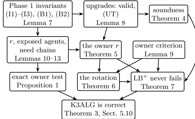
Fig. 3. How the results of Section 5 depend on each other. Theorems 1 and 2 follow from Theorem 7 with peeling (Section 5.8).
