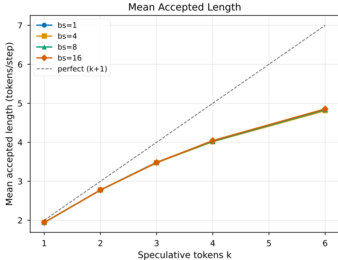
Plot 1 — Acceptance vs Speculative Depth (Qwen3.5-27B, MTP)
