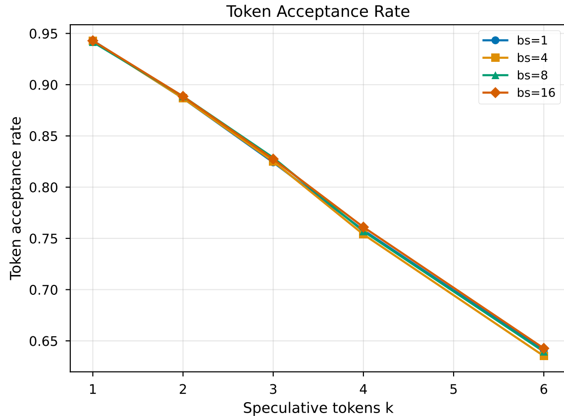
Plot 1 — Acceptance vs Speculative Depth (Qwen3.5-27B, MTP)
