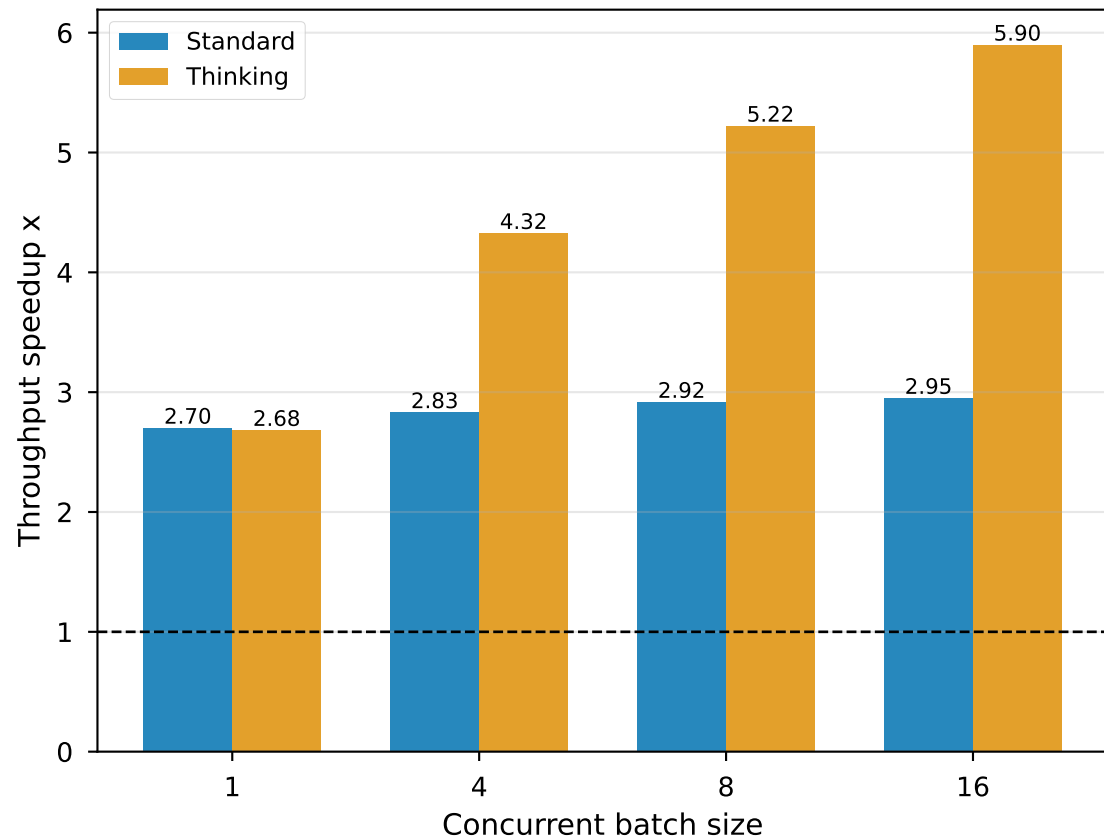
Plot 4 — Standard vs Thinking Mode (MoE 35B-A3B, MTP k=3)
