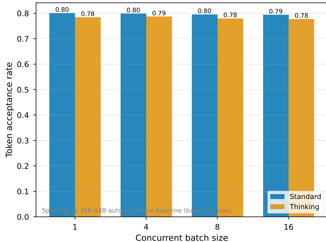
Plot 4 — Standard vs Thinking Mode (MoE 35B-A3B, MTP k=3)
