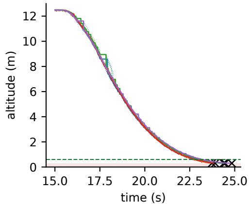
(a) goal 0.6 m, old Q_{ref}
