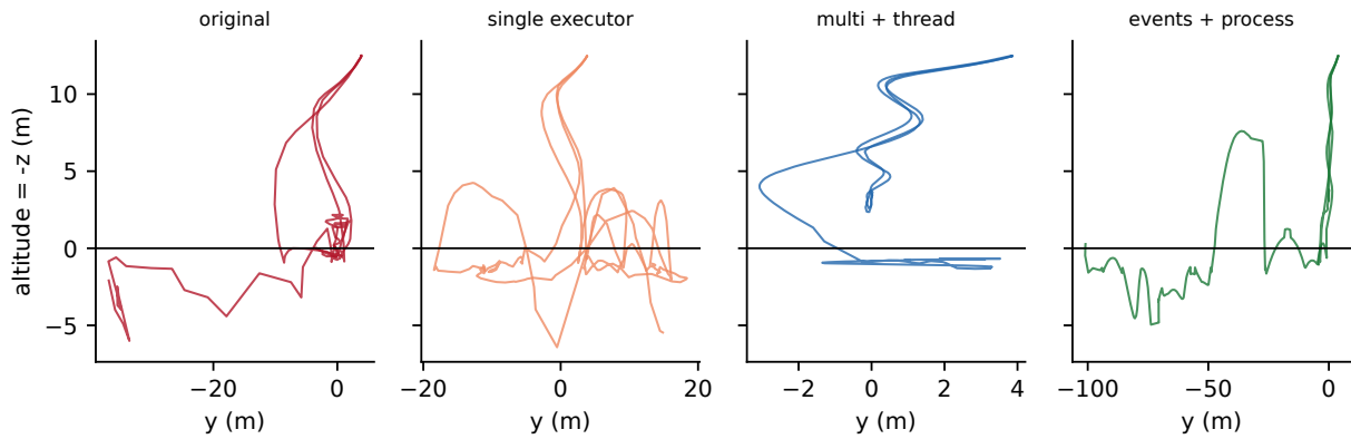
Figure 2: Flown paths in the y -altitude plane (three runs each, RTA phase). The black line is the ground.
