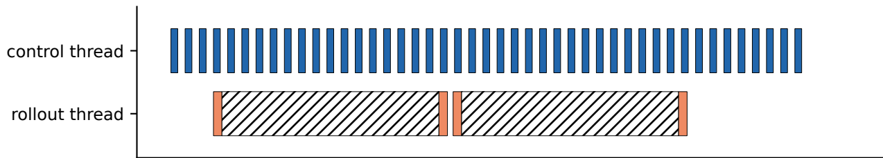
(c) EventsExecutor + ProcessRolloutBackend
