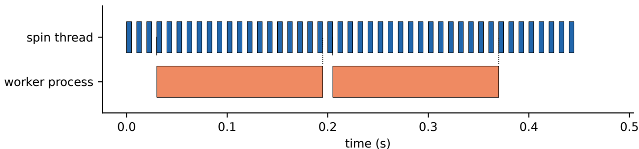
(c) EventsExecutor + ProcessRolloutBackend
