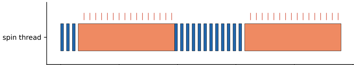
(b) MultiThreadedExecutor + separate callback groups (thread backend)
