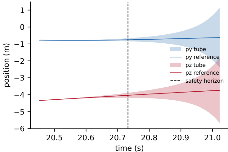
(b) plan #27: stored tube until it is 4 m wide
