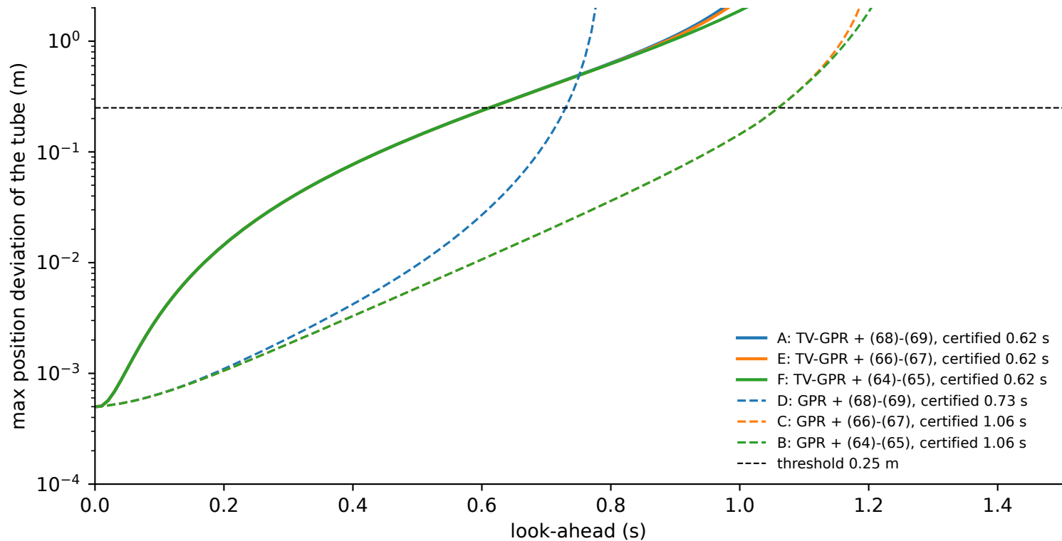
plan #18 ( t = 9.8 s), same inputs, six tubes (solid TV-GPR, dashed GPR)
