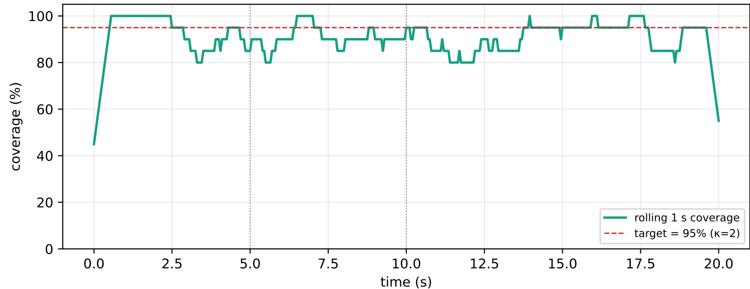
Estimator coverage over time (overall = 91.8%)
