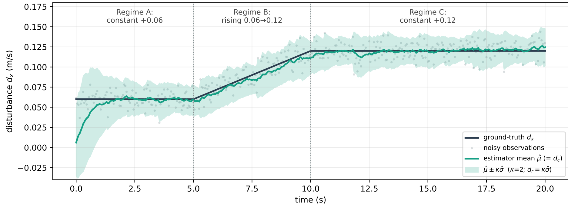
Online EWMA disturbance estimator on a 3-regime trace — coverage = 91.8%
