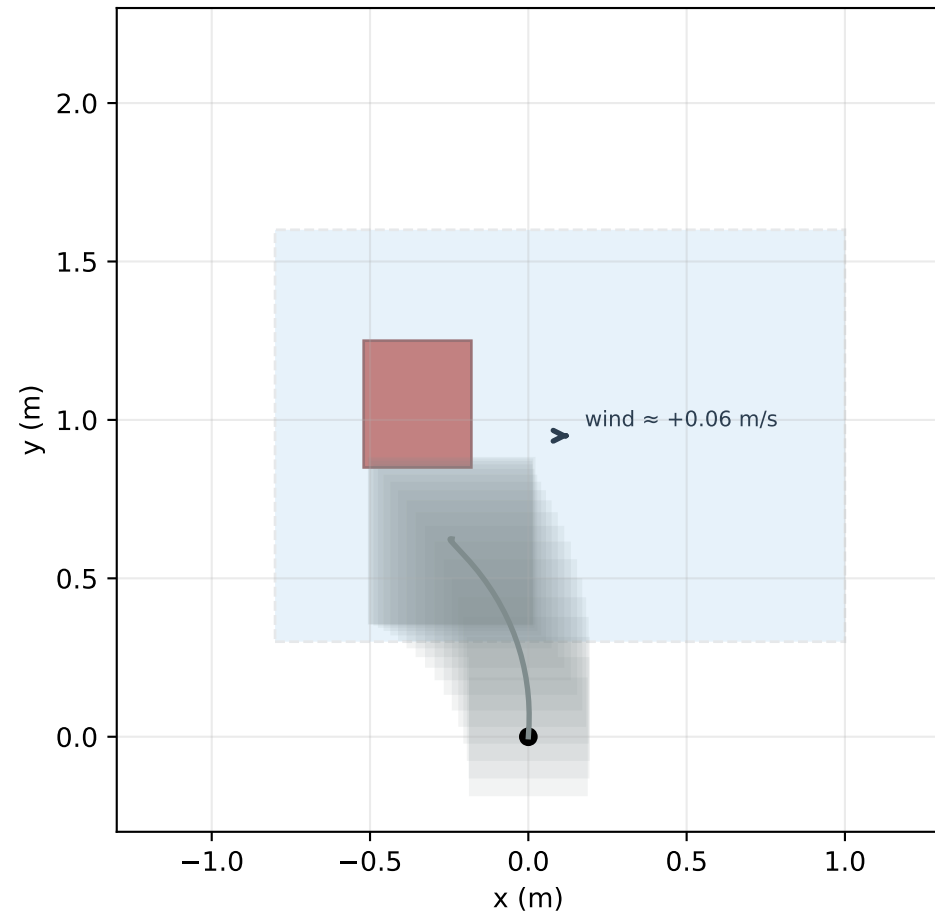
goal-only (no MMR) k = (1.0, 0.28) , hard m_{dir} = -0.032 , m_{sym} = -0.032 \rightarrow UNSAFE
