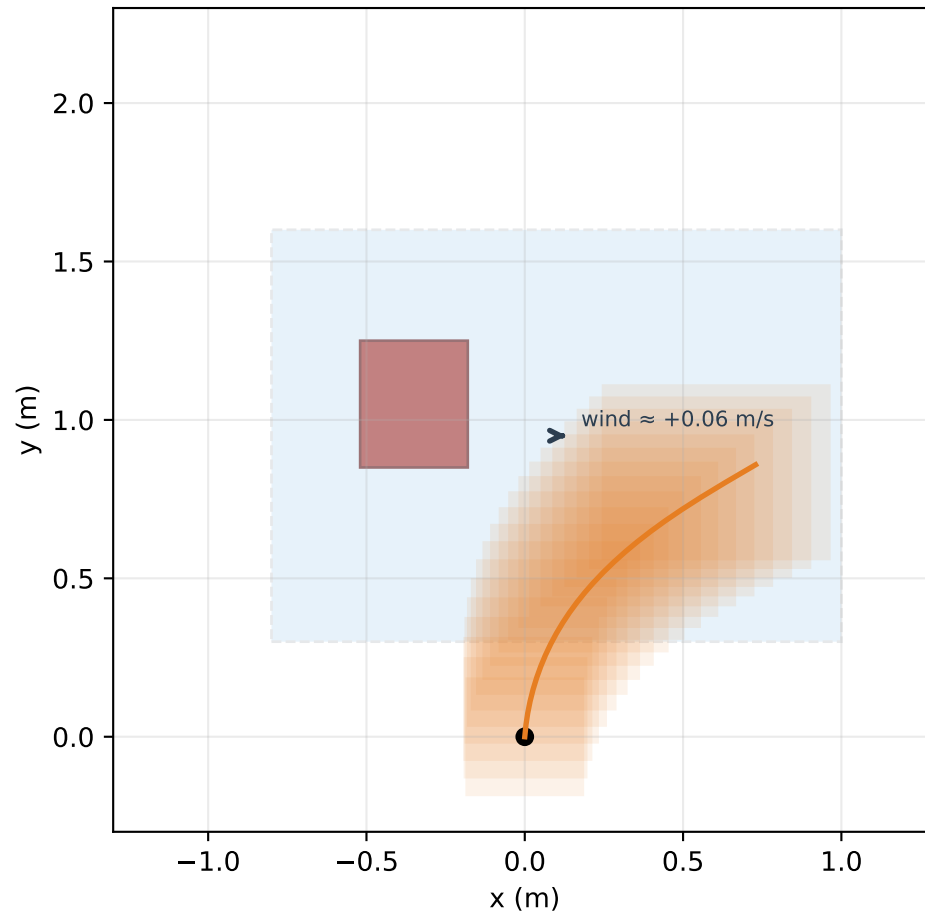
goal + symmetric MMR constraint k = (-1.0, -1.0) , hard m_{dir} = +0.167 , m_{sym} = +0.115 \rightarrow safe
