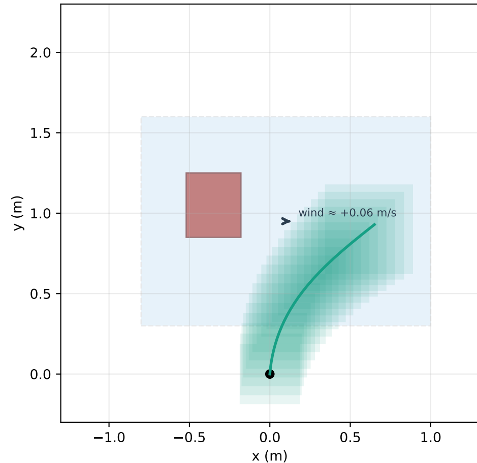
goal + directional MMR constraint k = (-0.85, -1.0) , hard m_{dir} = +0.145 , m_{sym} = +0.089 \rightarrow safe
