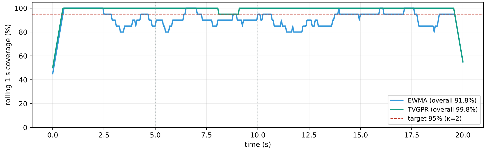
Coverage over time: TVGPR vs EWMA
