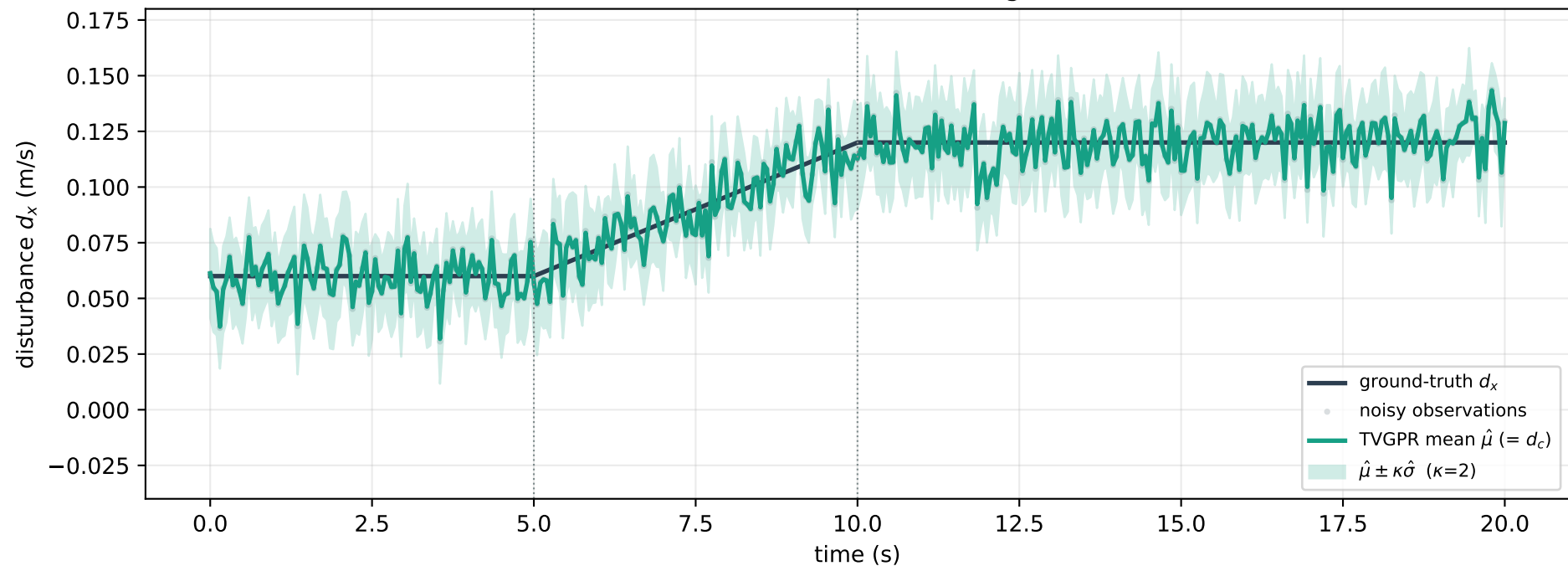
TVGPR online estimator — coverage = 99.8%
