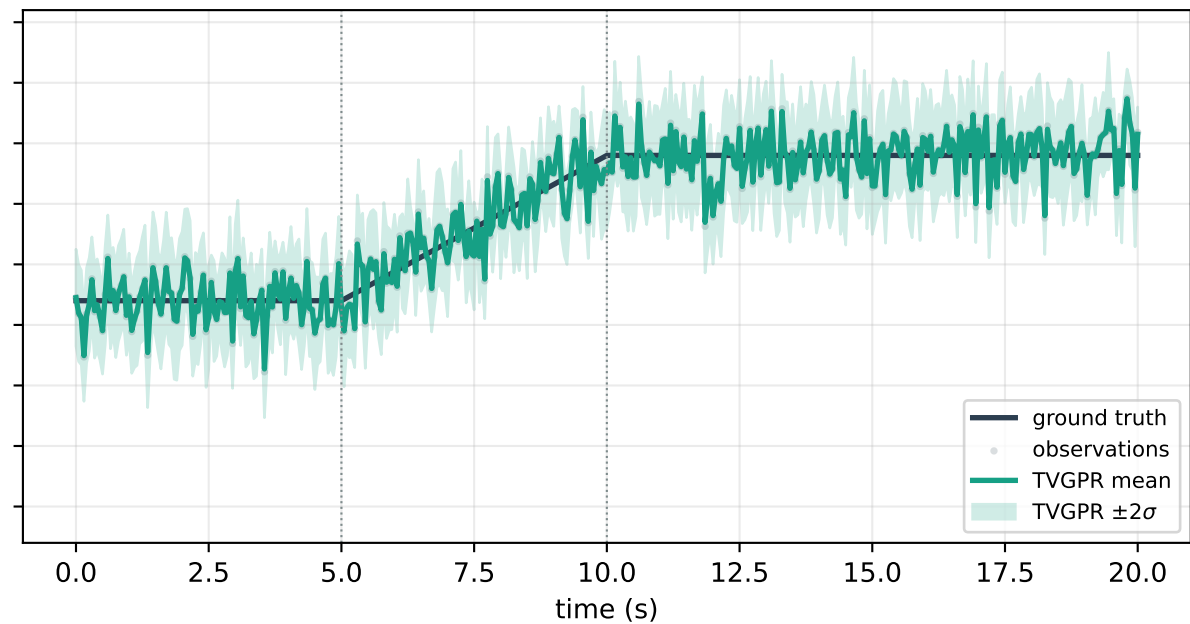
TVGPR — coverage = 99.8%
