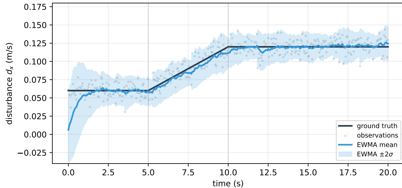
EWMA — coverage = 91.8%
