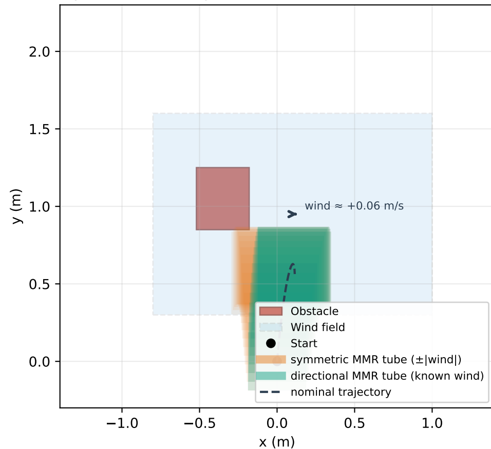
Initial k = (-0.12, 0.85) symmetric (orange) vs directional (teal) MMR tubes
