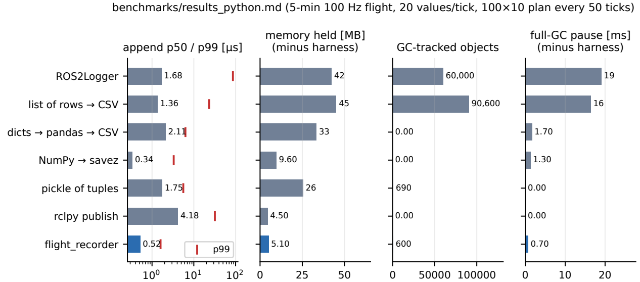
Figure 8: The recorded benchmark results. Memory and full-GC pause are shown after subtracting the harness (noop: 5.1 MB, 10.0 ms). The red ticks on the first panel mark p99.
