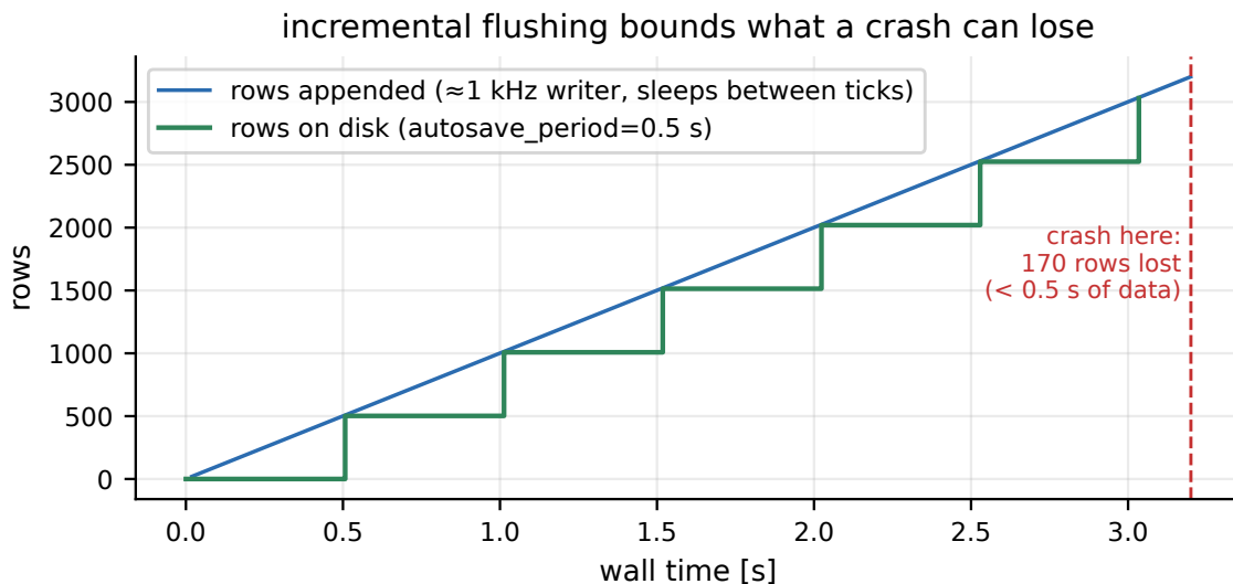
Figure 6: Rows appended by a writer at about 1 kHz (sleeping between ticks, like an rcply timer) against rows safely on disk with autosave_period=0.5 . The flushes happen on the recorder's background thread. If the process died at the red line, everything below the green staircase would survive.
