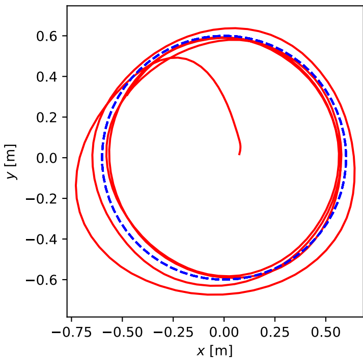
a) JAX: Circle Horz 2x RMSE = 91.22 cm
