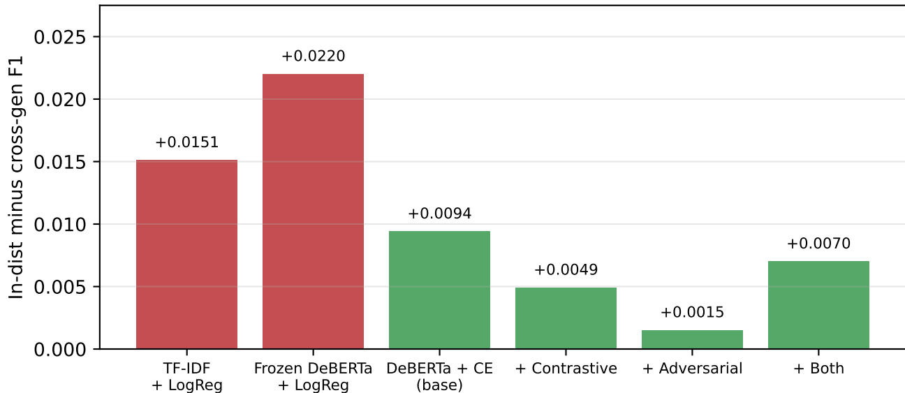
Cross-generator generalization gap (lower is better)
