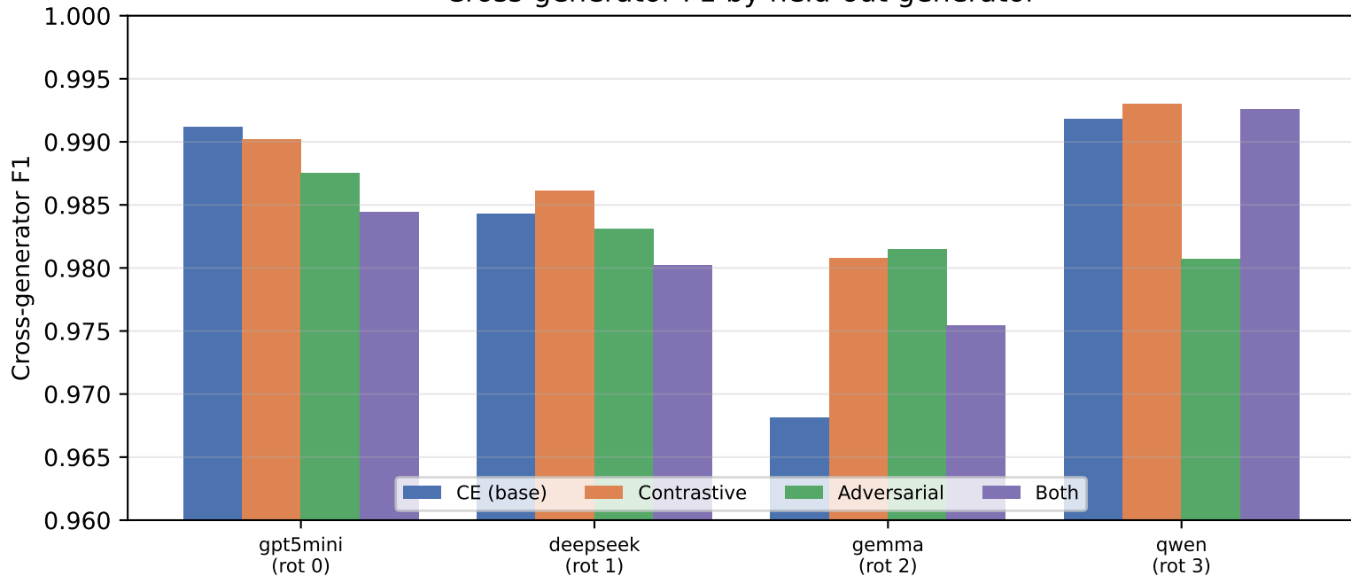
Cross-generator F1 by held-out generator
