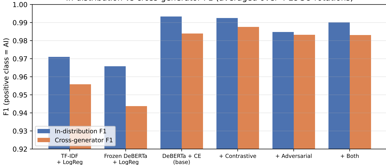
In-distribution vs cross-generator F1 (averaged over 4 LOGO rotations)
