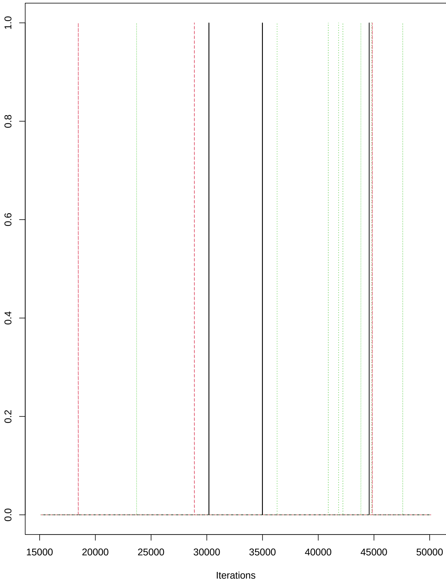
Trace of z[1,4,2]
