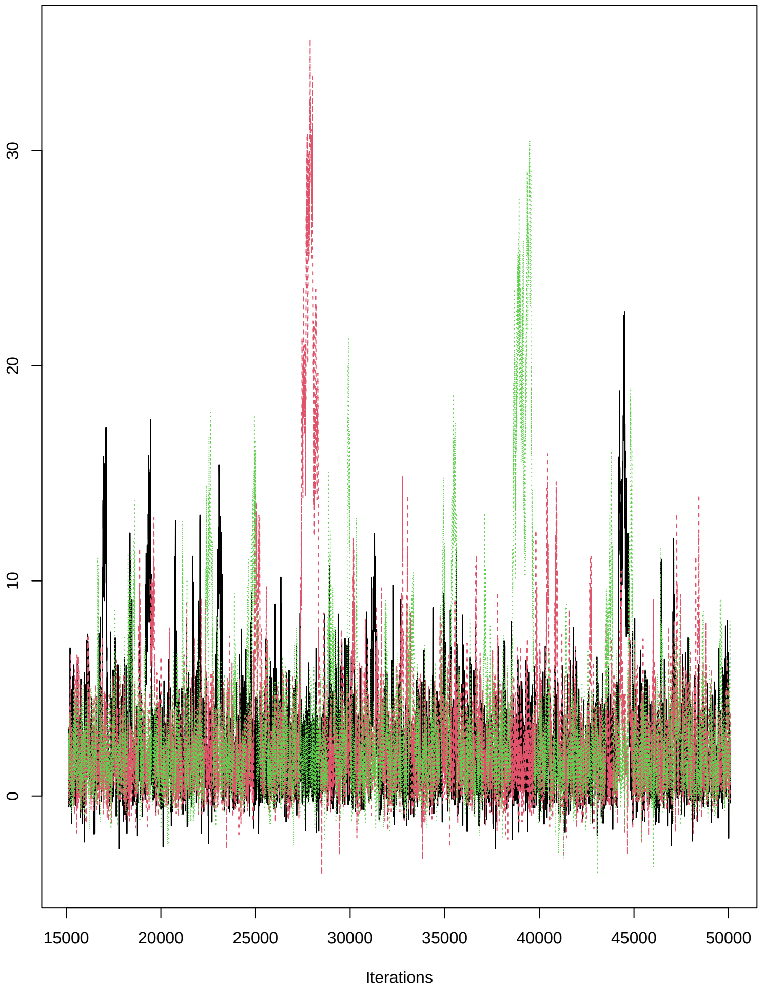
Trace of land_re[2]
