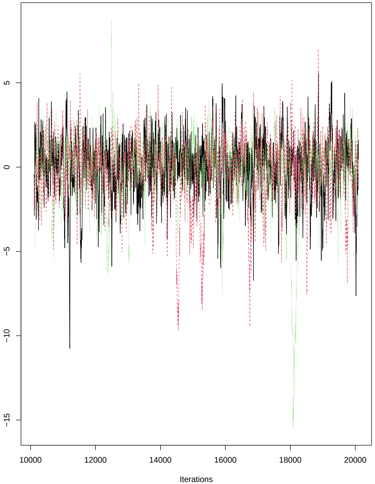
Trace of beta_yr_egg[3]
