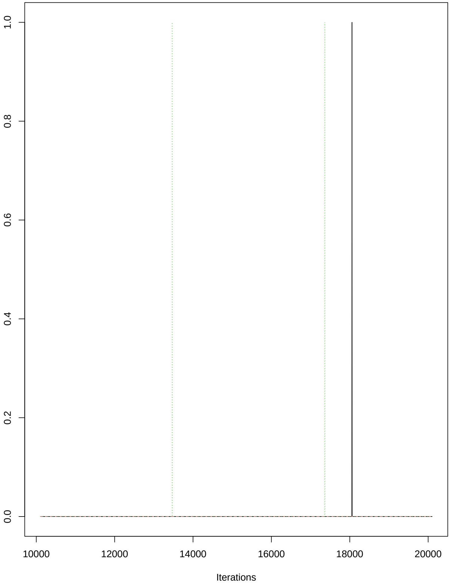
Trace of z[1,3,2]
