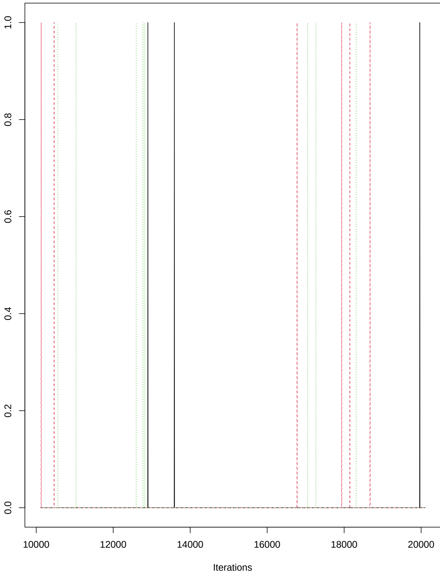
Trace of z[1,9,2]
