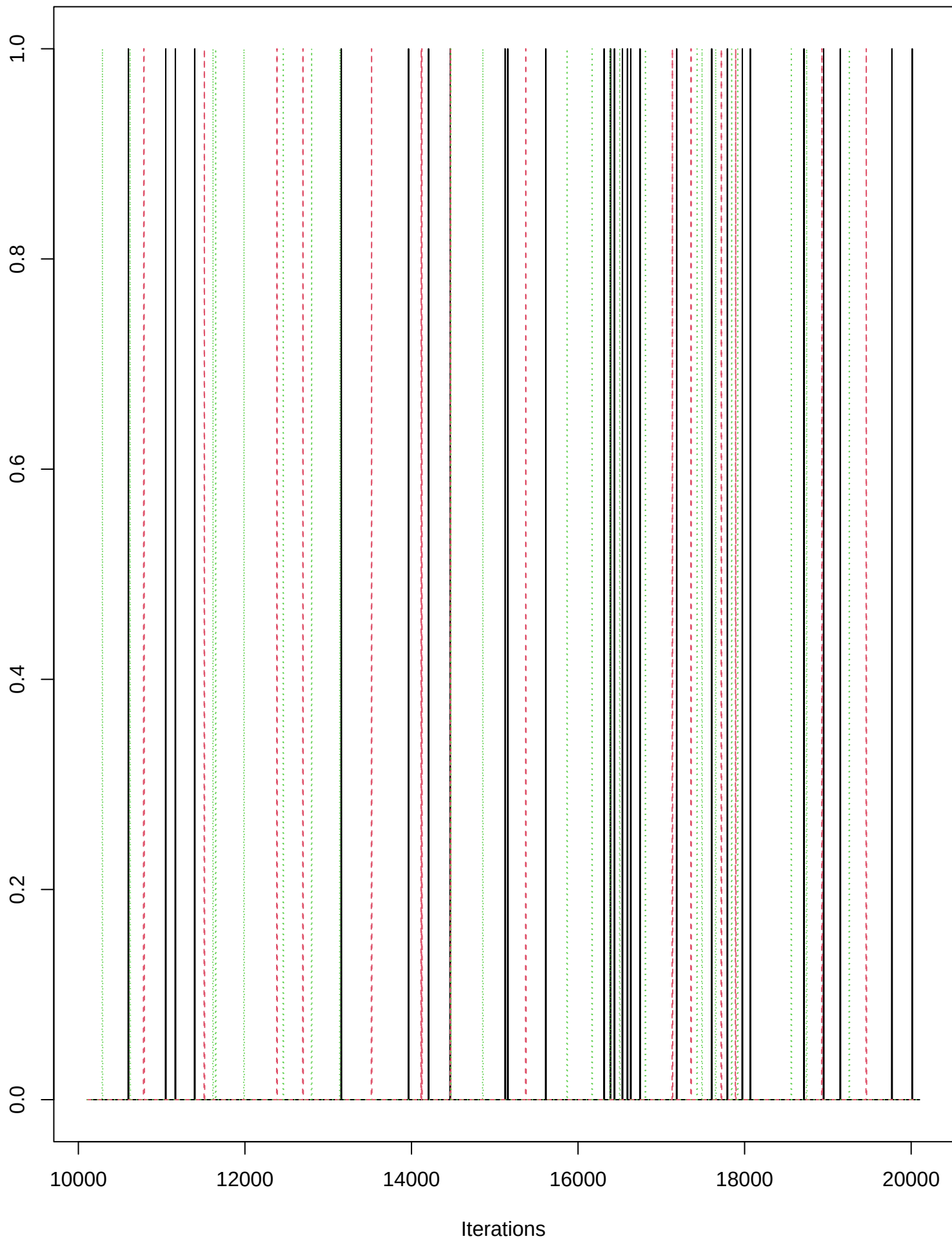
Trace of z[1,4,3]
