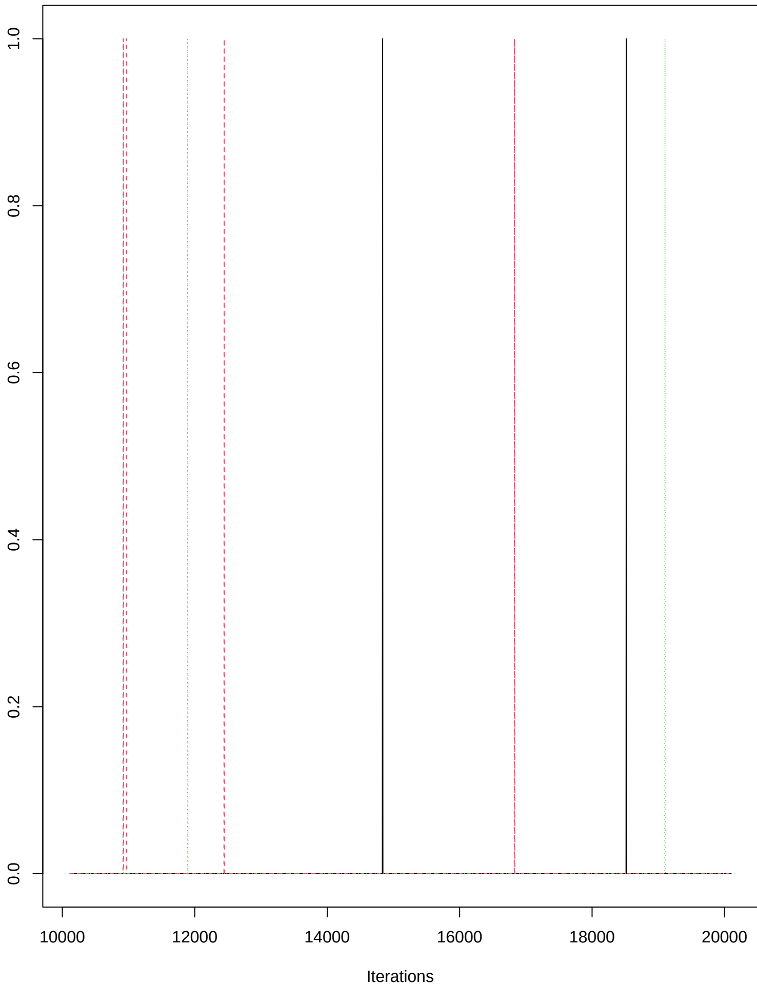
Trace of z[1,8,2]
