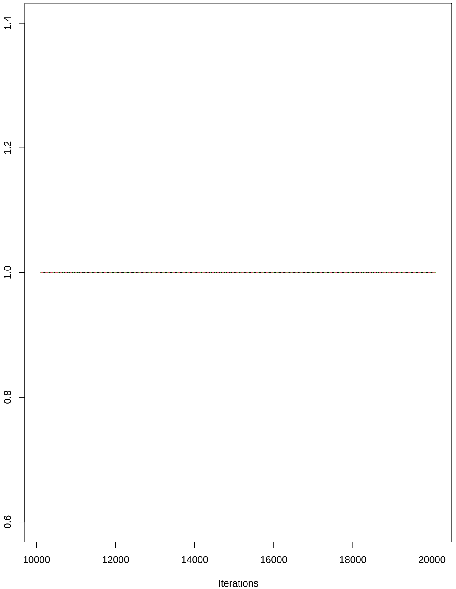
Trace of z[1,6,3]
