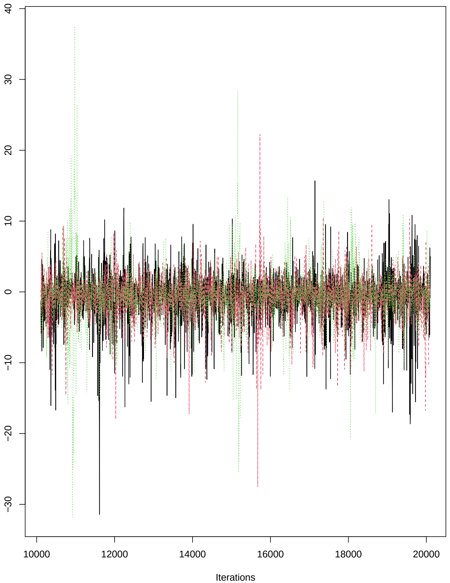
Trace of beta_mon_egg[6]
