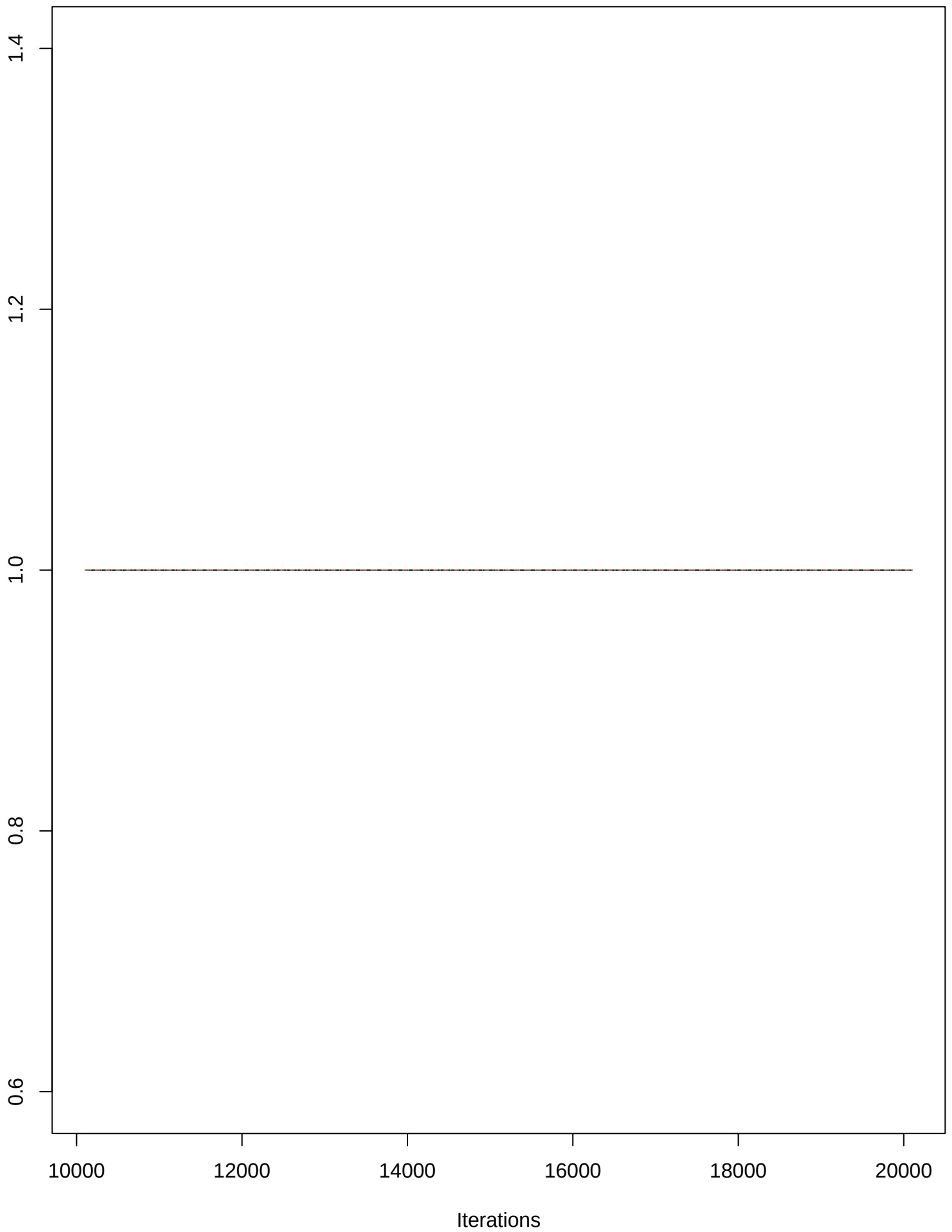
Trace of z[2,10,2]
