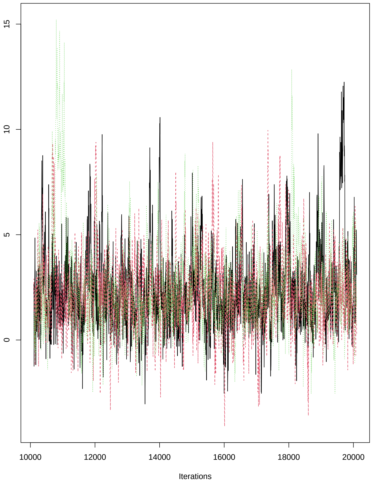
Trace of beta_mon_egg[2]
