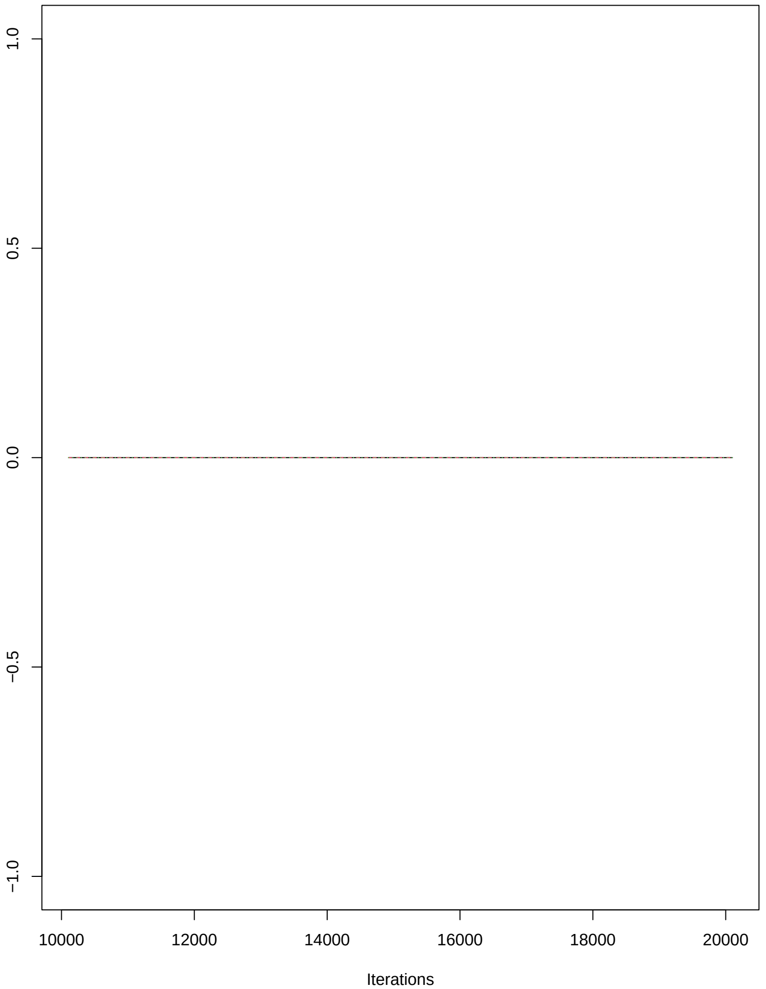
Trace of z[1,4,2]
