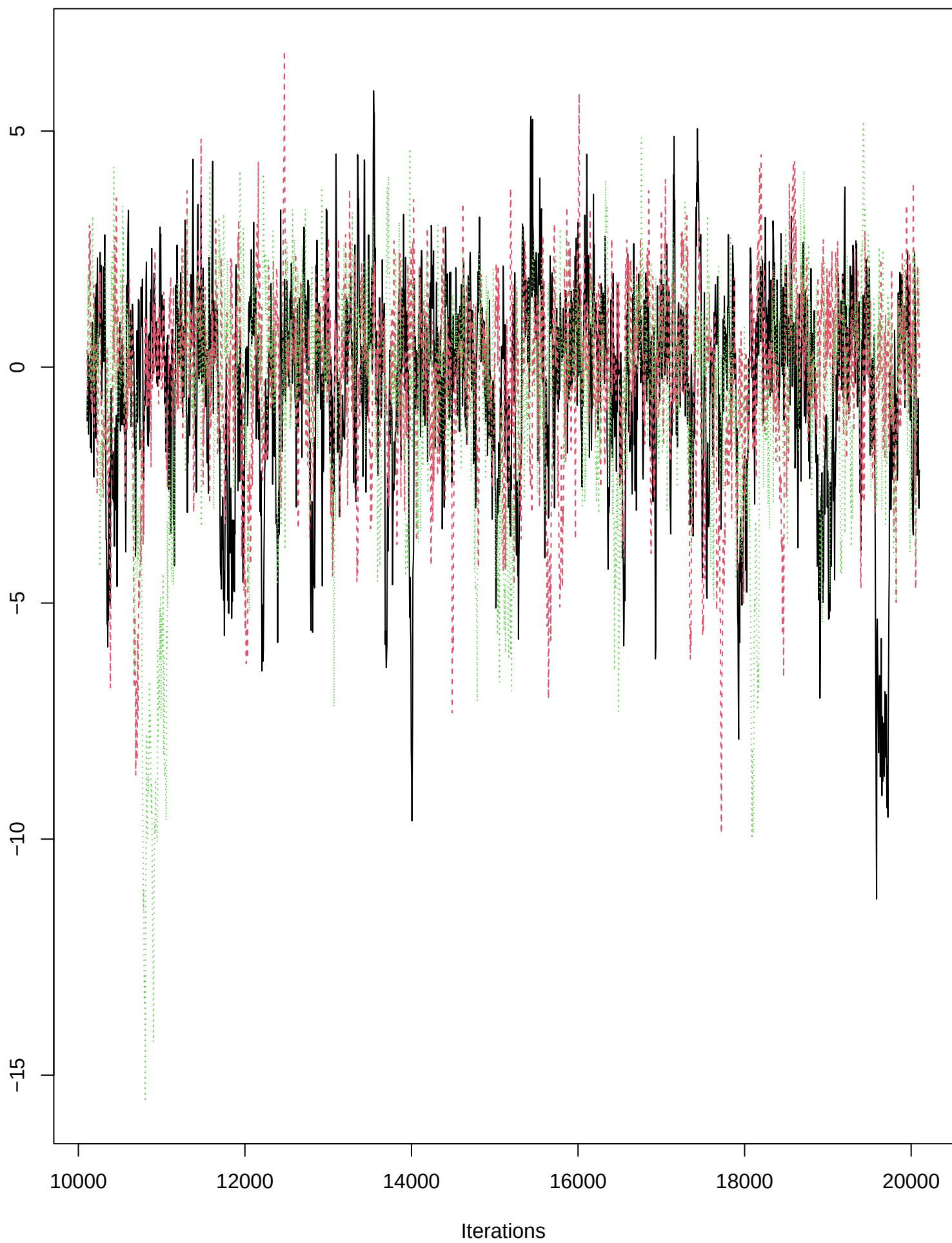
Trace of beta_yr_egg[3]
