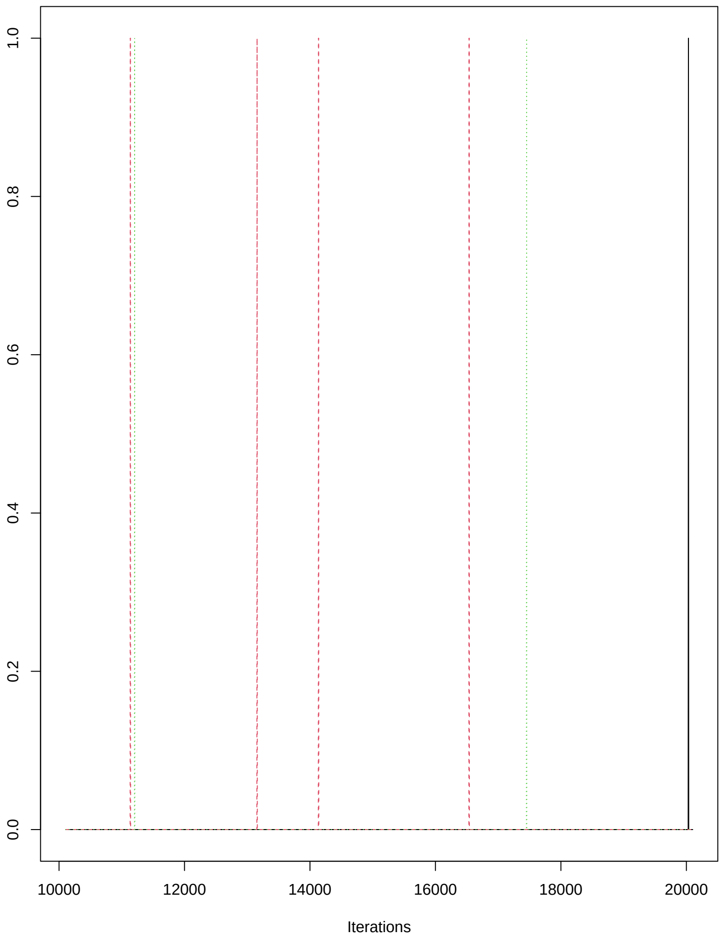
Trace of z[1,13,2]
