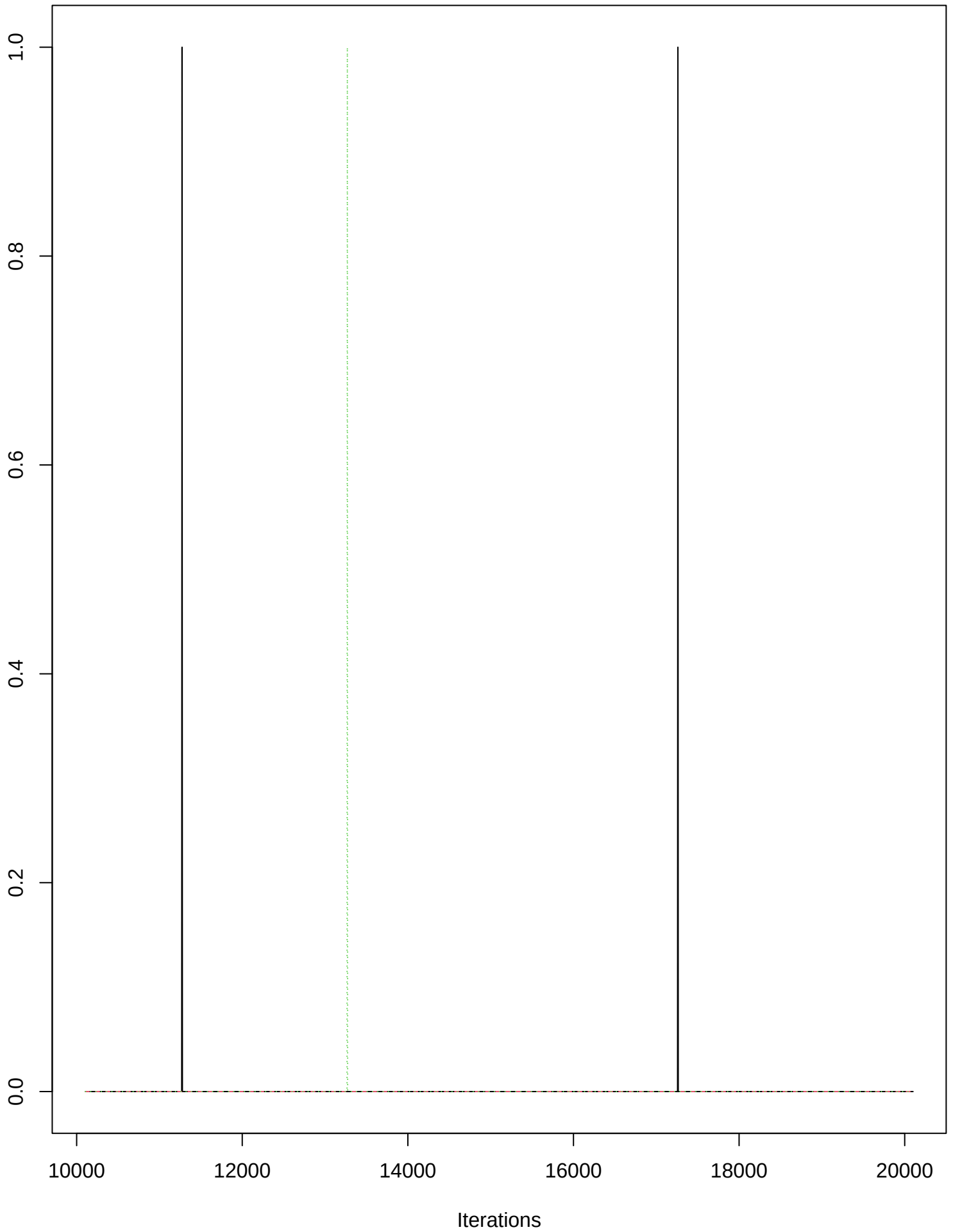
Trace of z[1,2,2]
