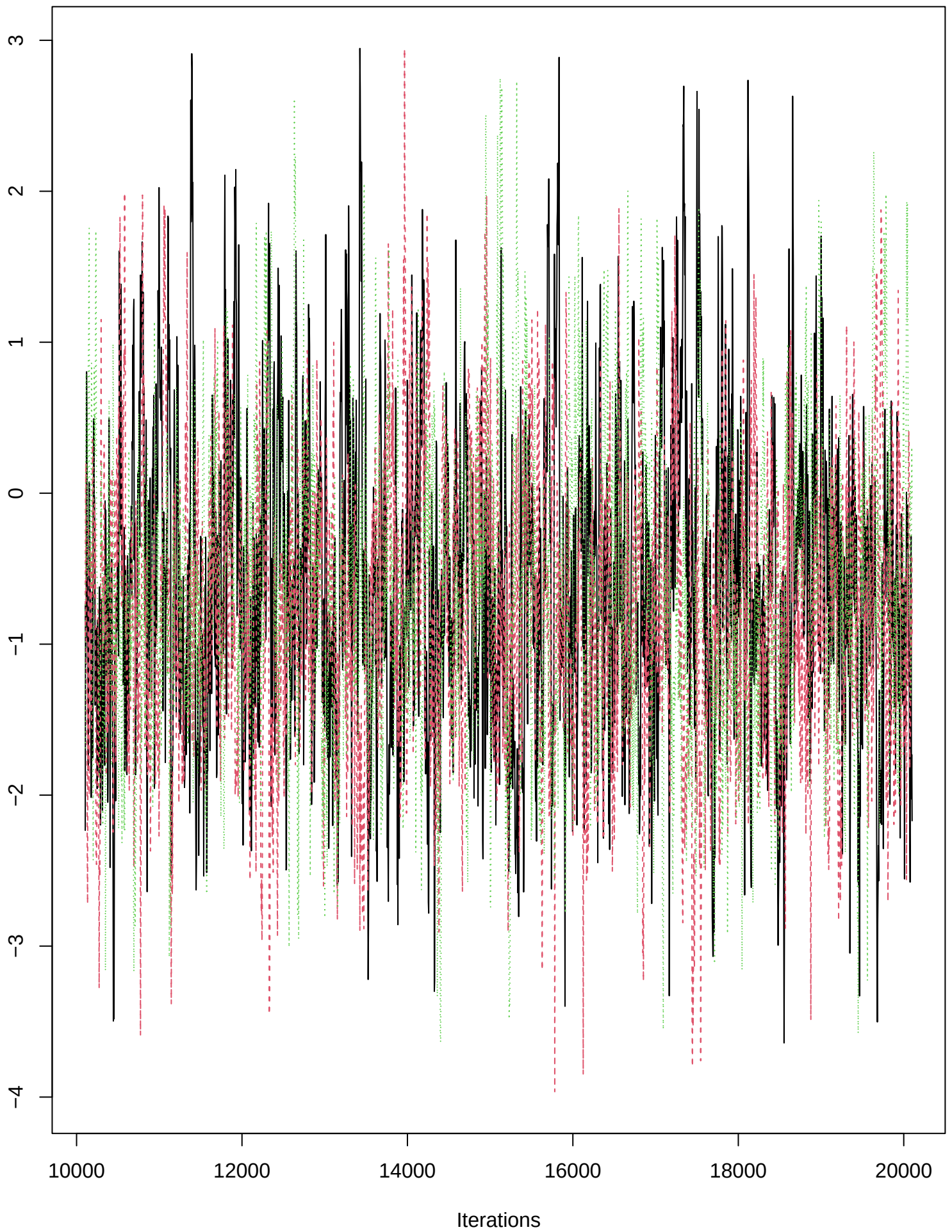
Trace of beta0_dip
