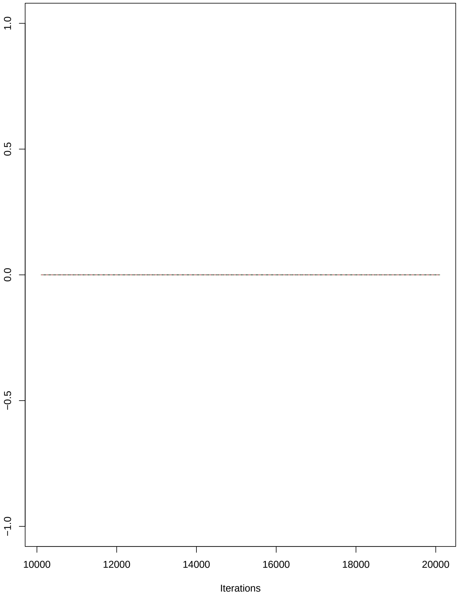
Trace of z[1,6,2]
