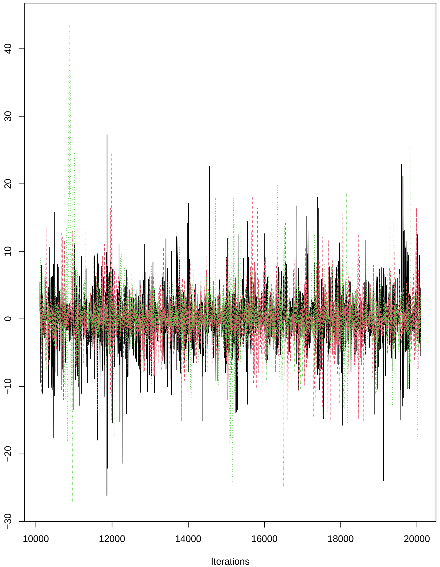
Trace of beta_mon_egg[8]
