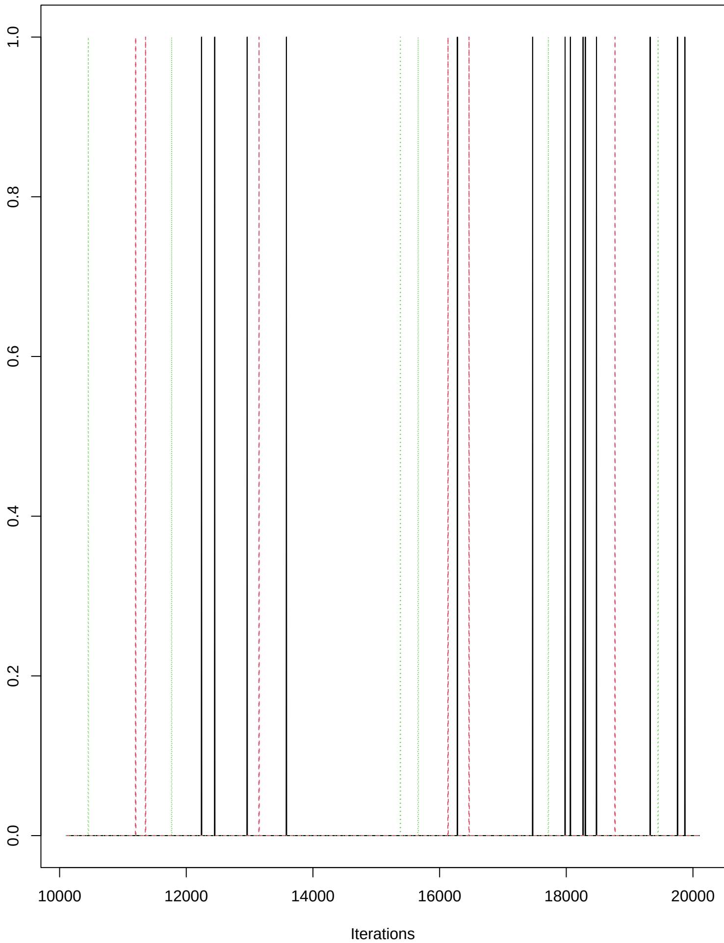
Trace of z[1,7,2]
