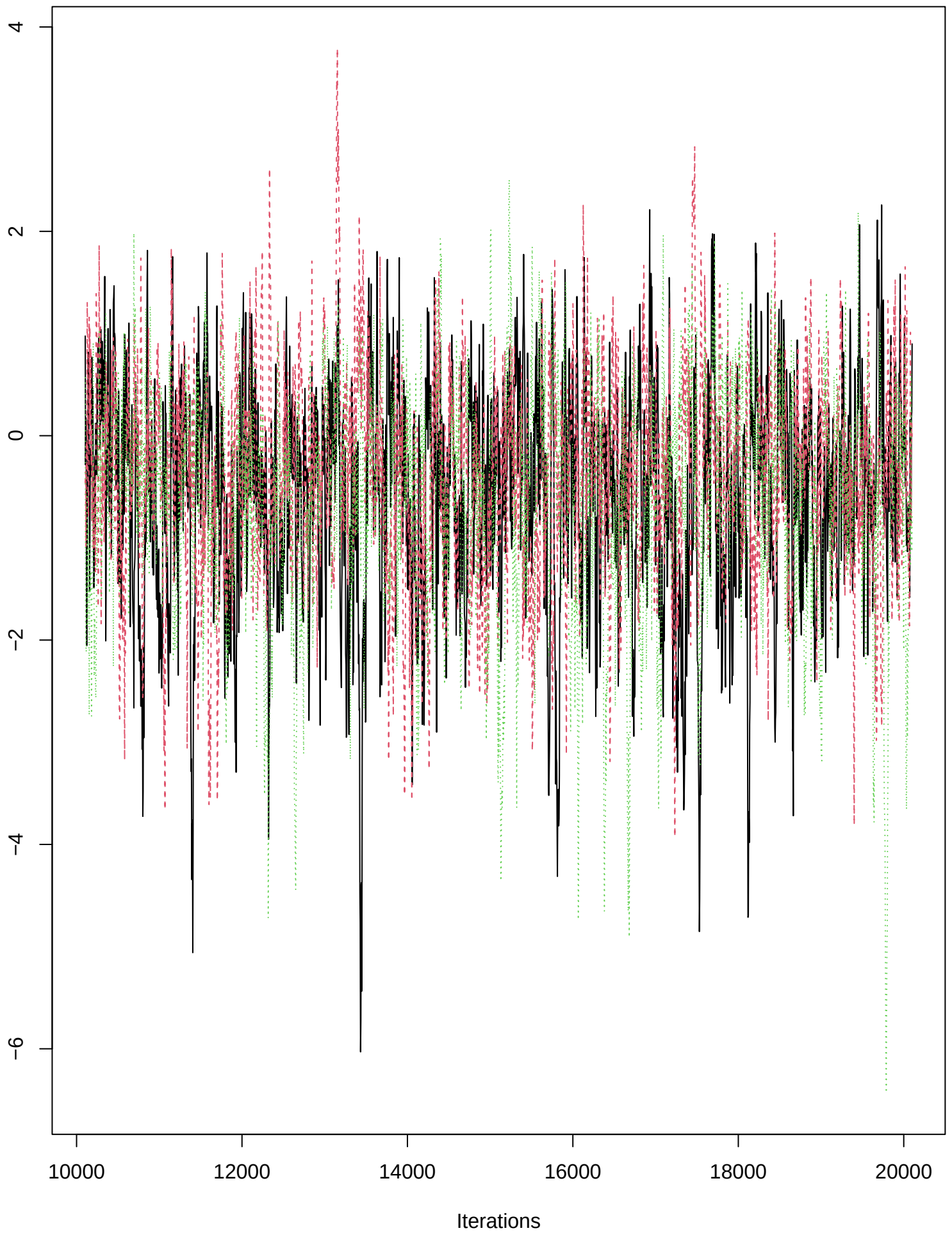
Trace of beta_yr_dip[3]
