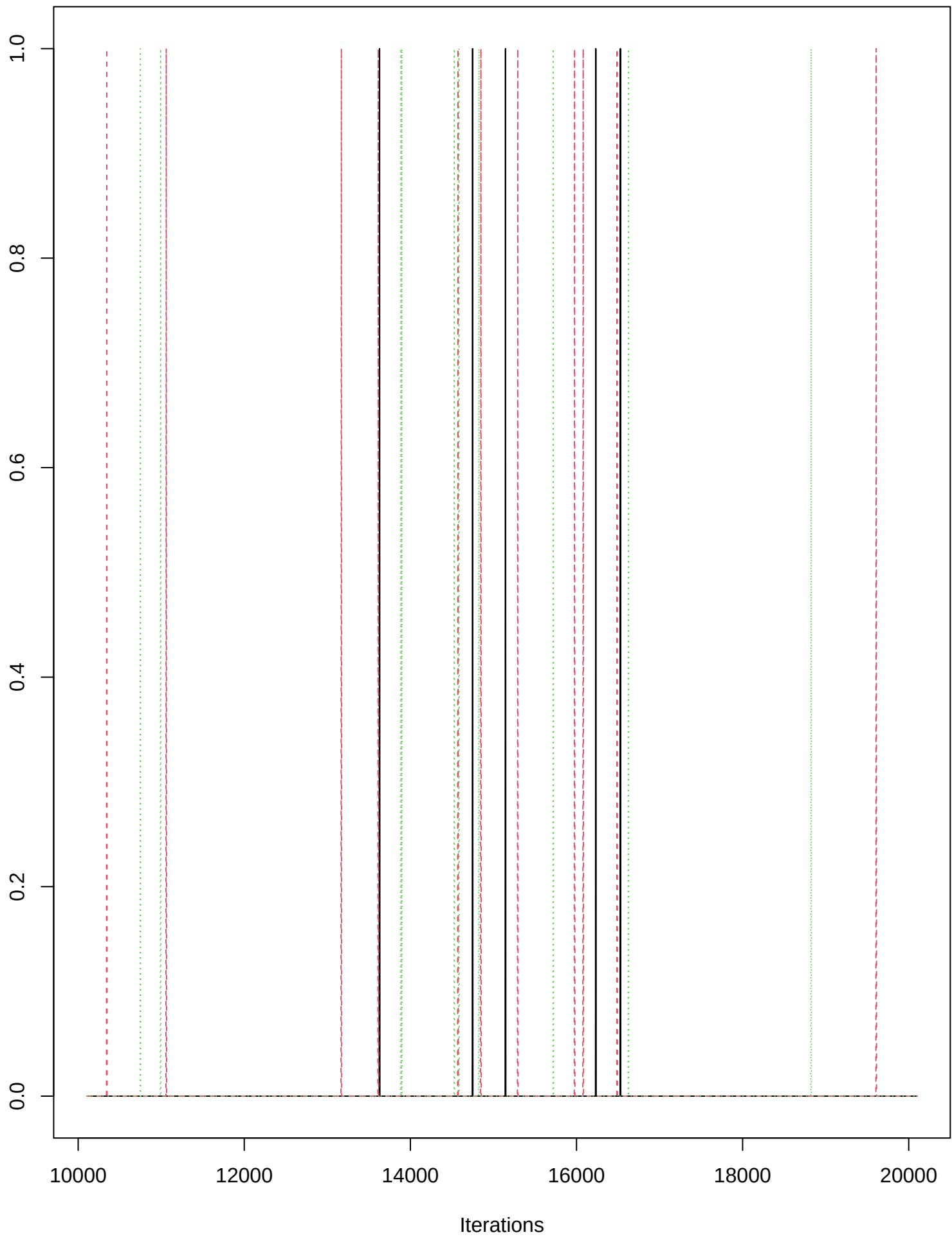
Trace of z[1,2,3]
