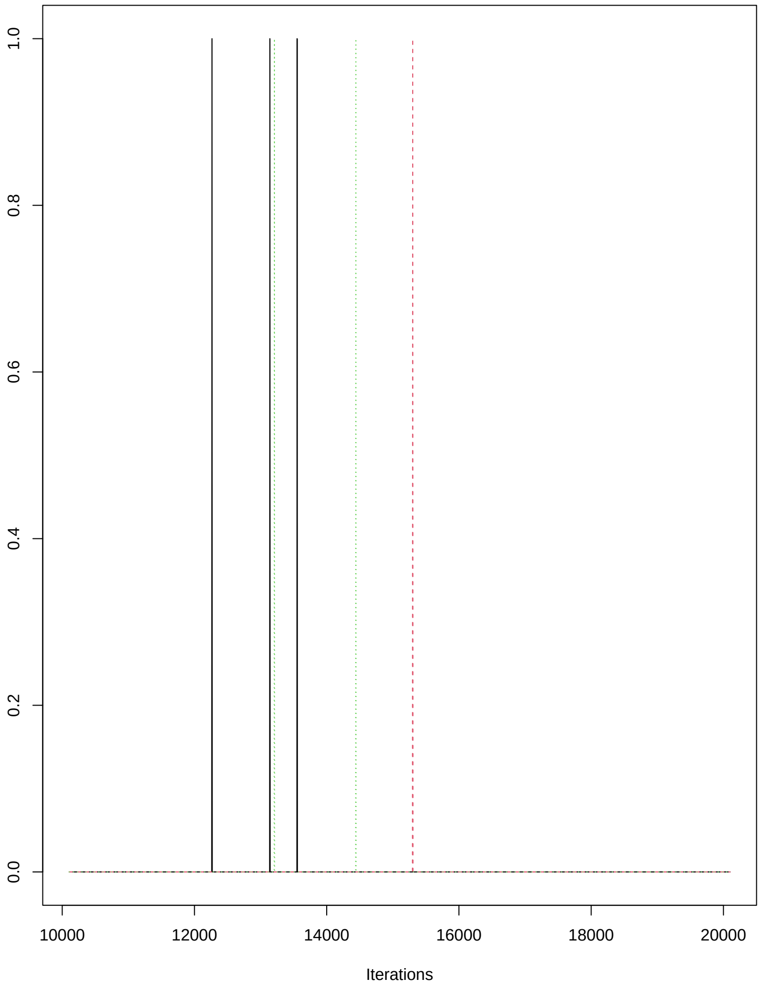
Trace of z[1,8,2]
