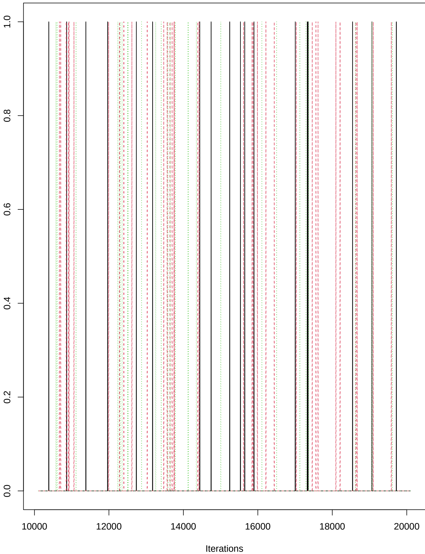
Trace of z[2,6,2]
