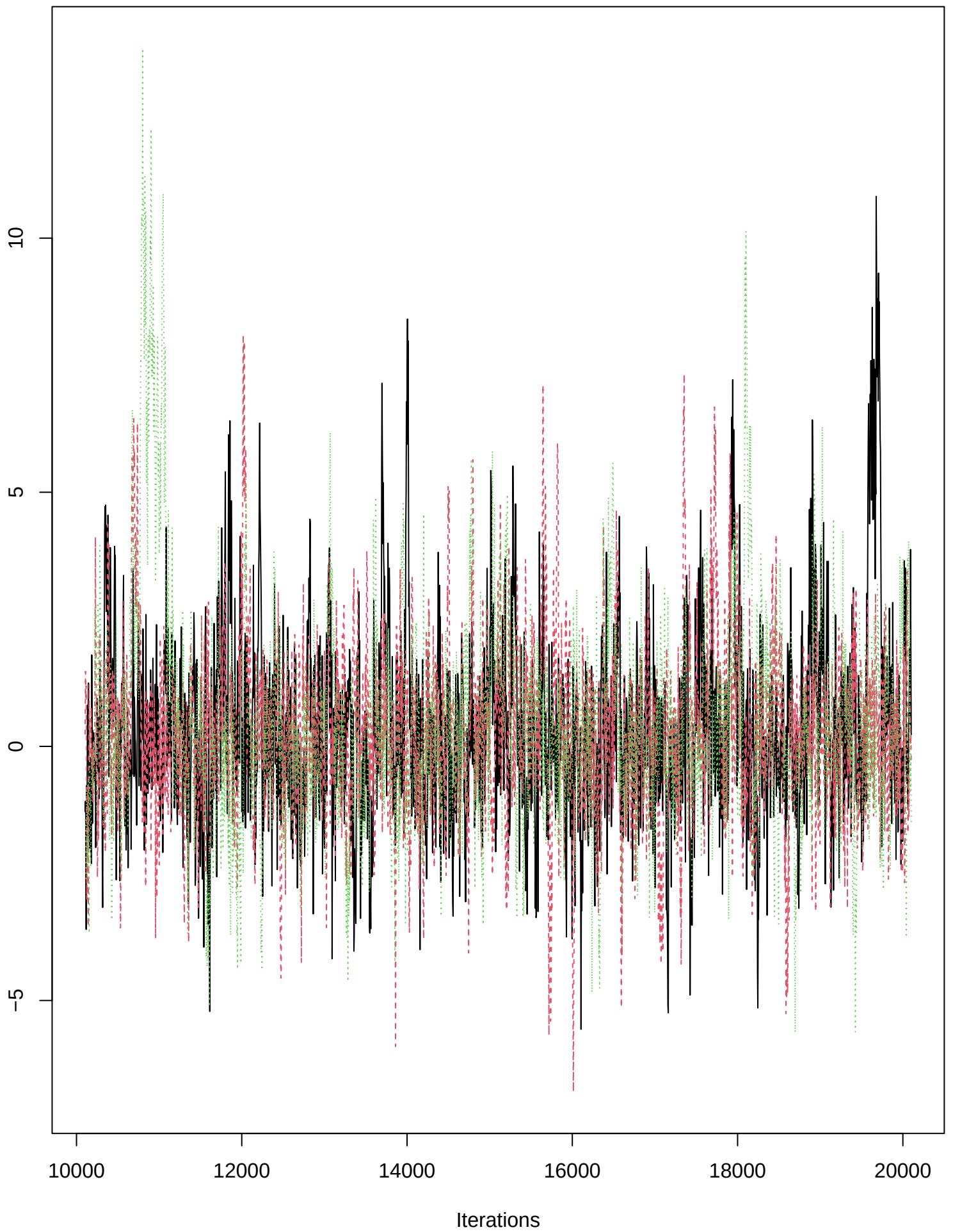
Trace of beta_mon_egg[3]
