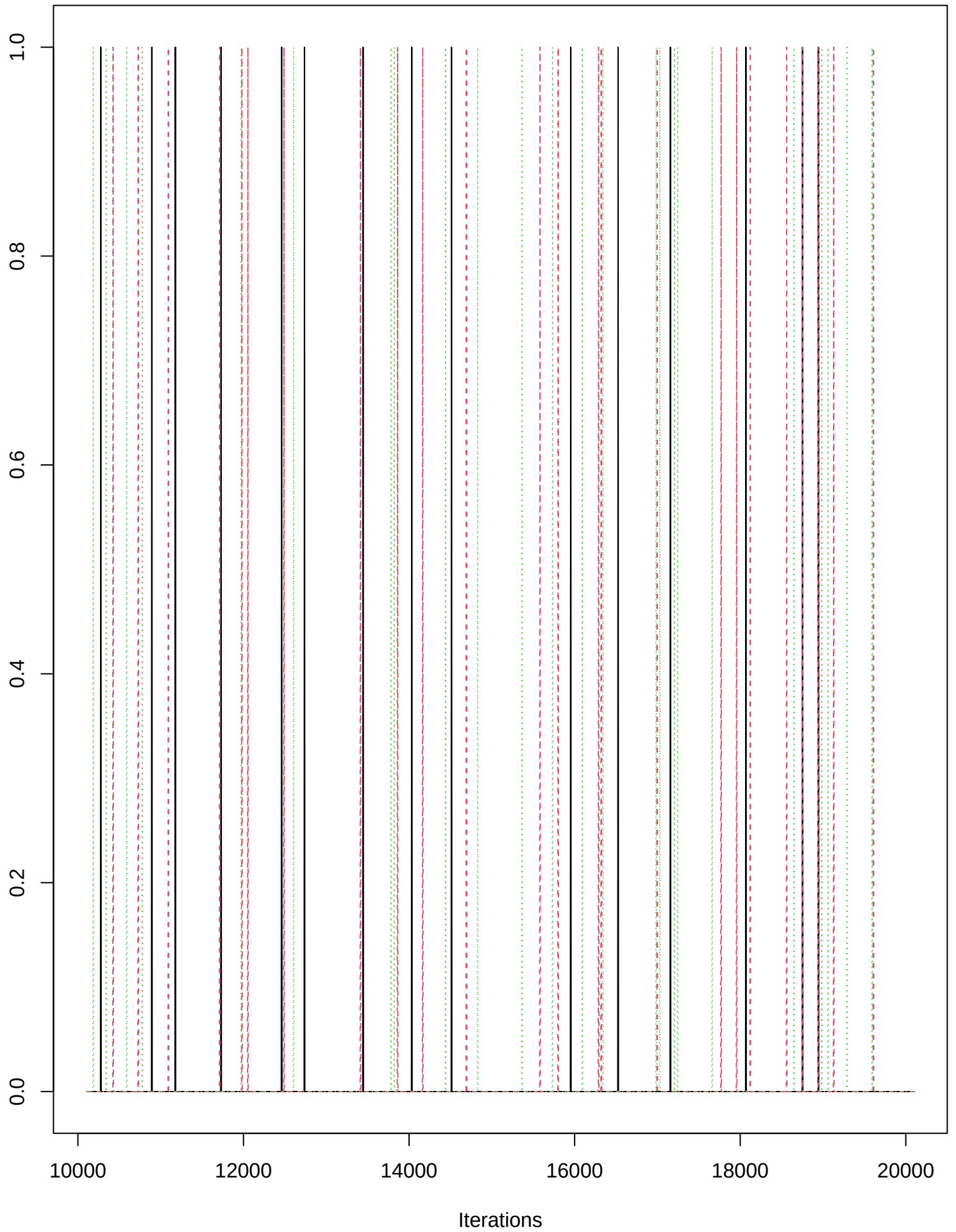
Trace of z[1,8,3]
