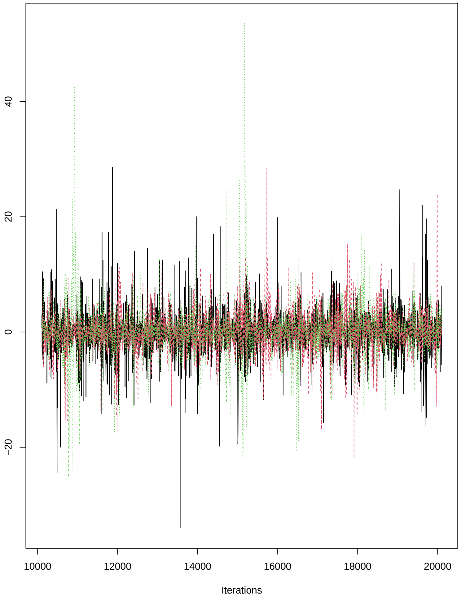
Trace of beta_yr_egg[1]
