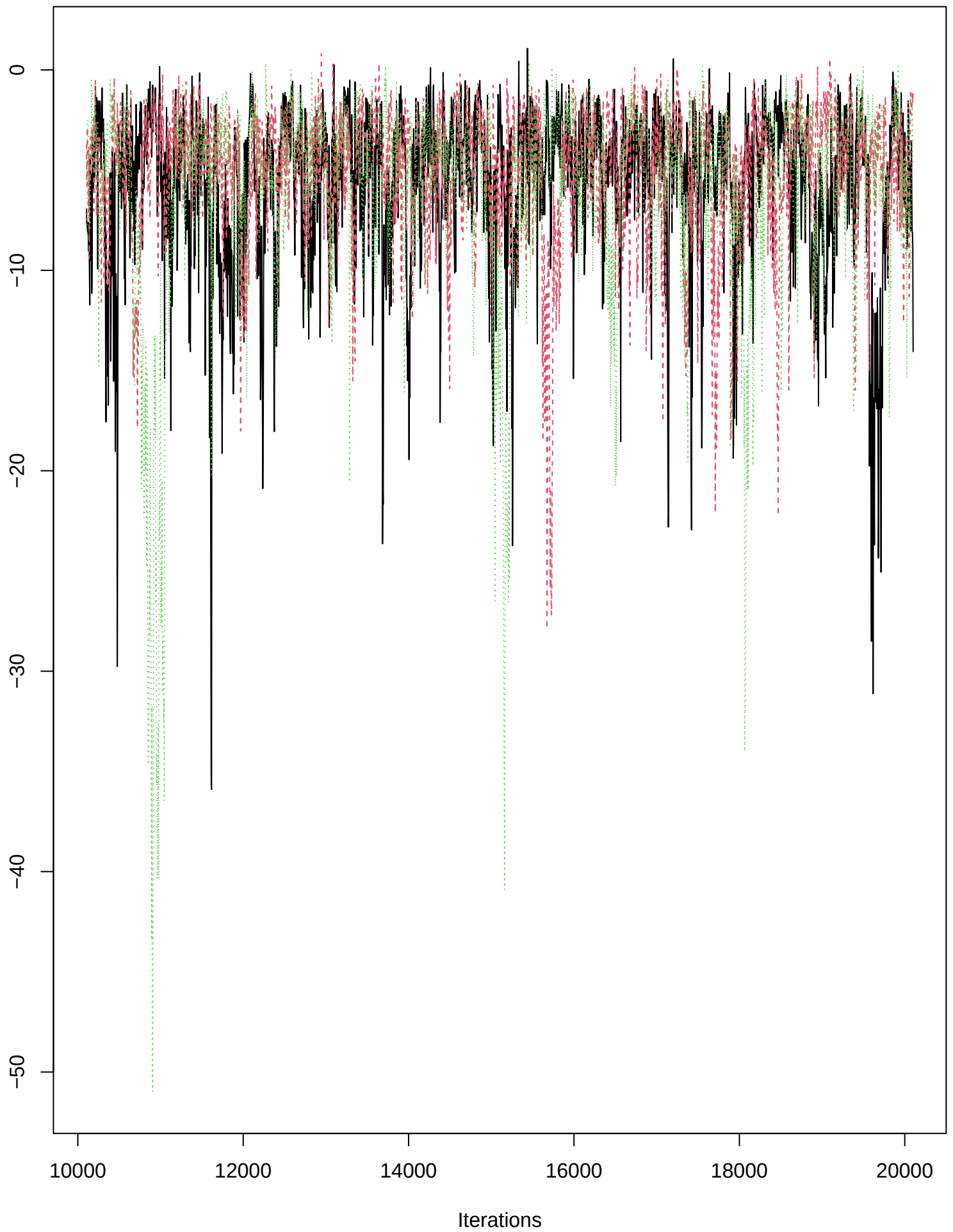
Trace of beta_yr_egg[2]
