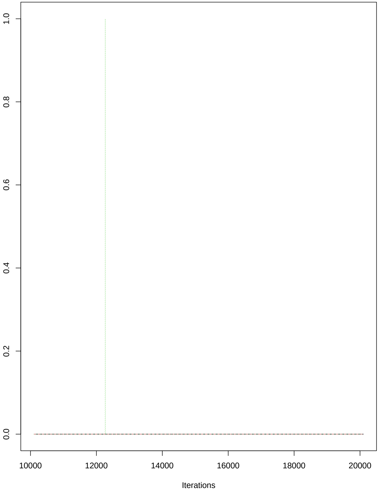
Trace of z[1,1,2]
