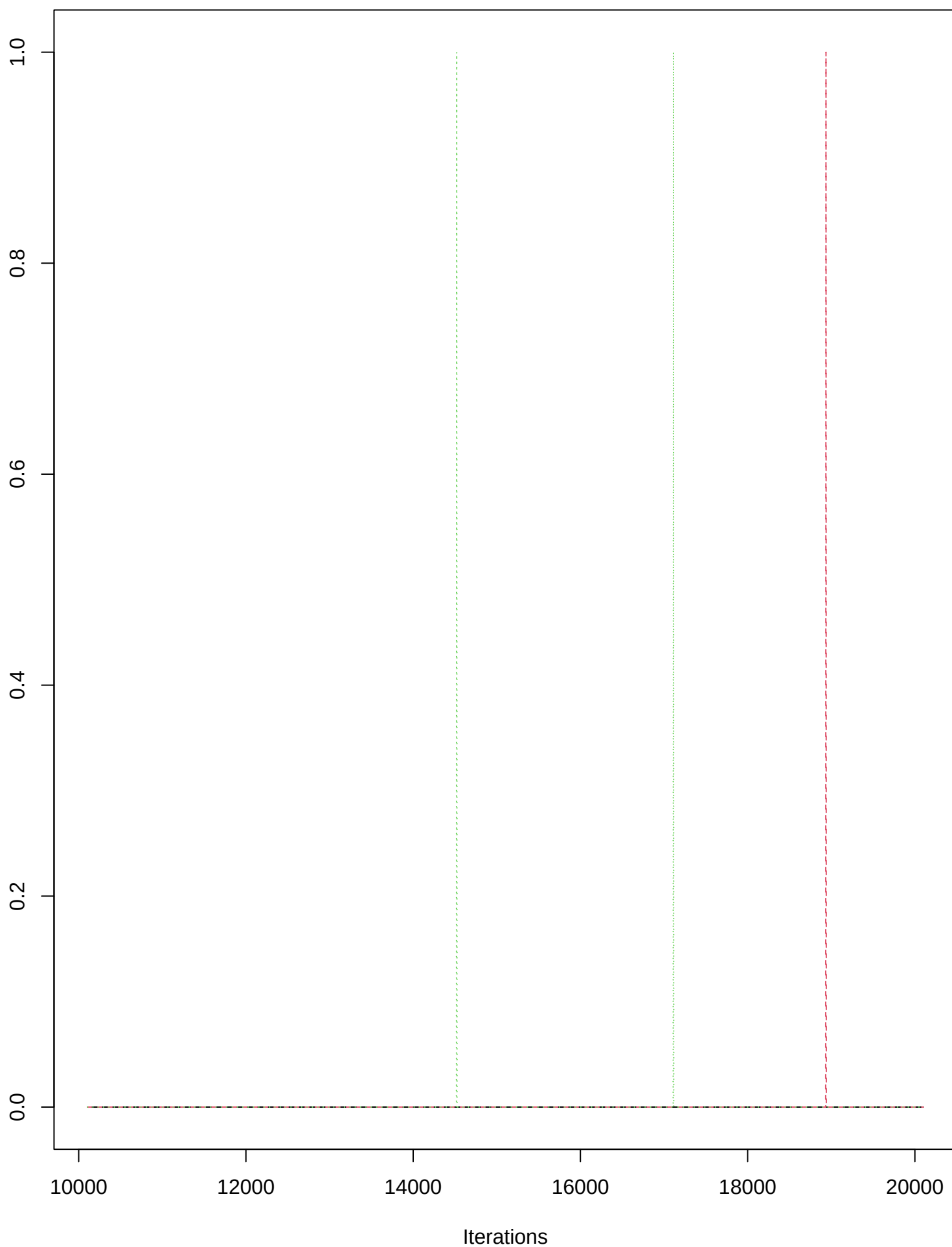
Trace of z[1,3,2]
