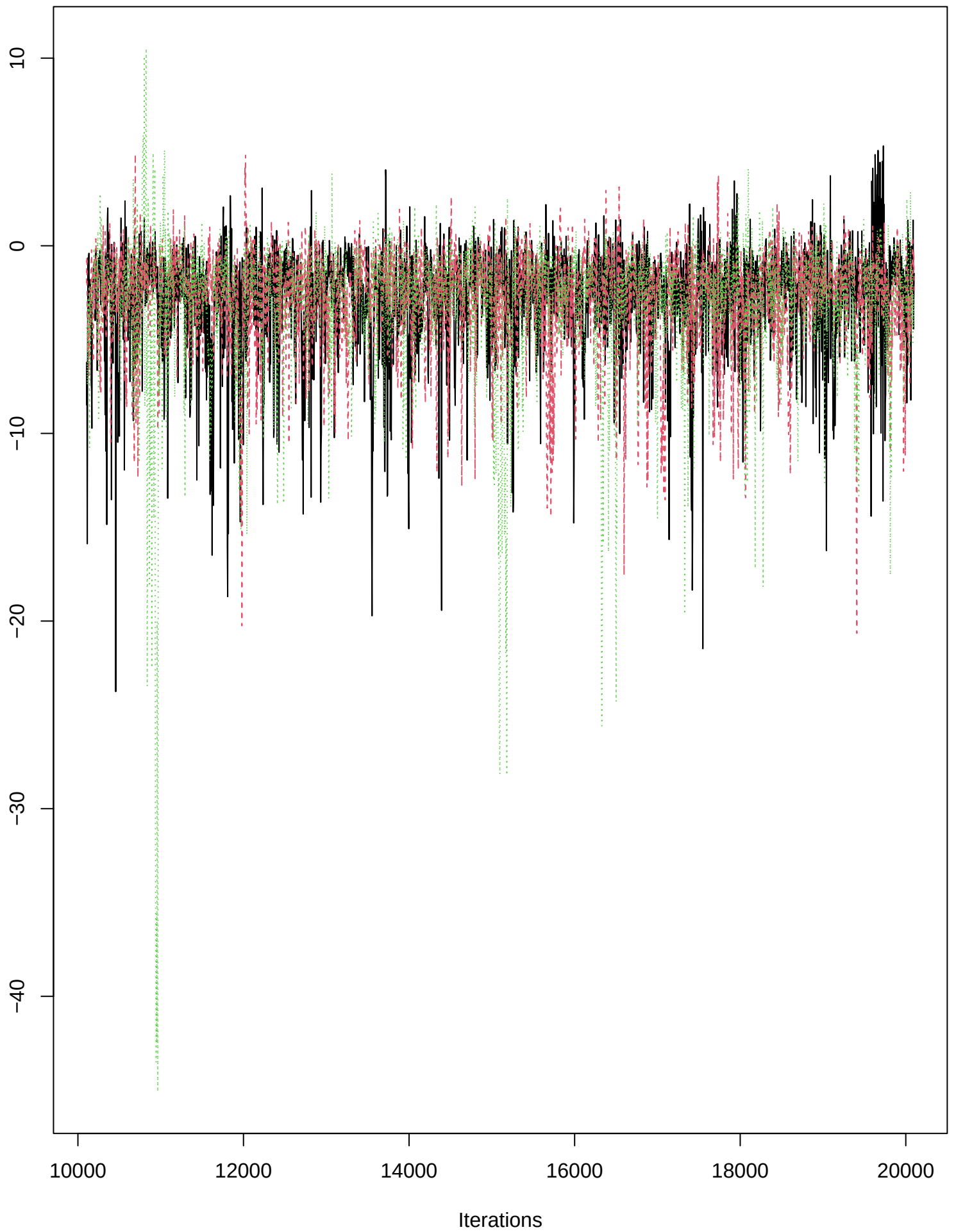
Trace of beta_mon_egg[4]
