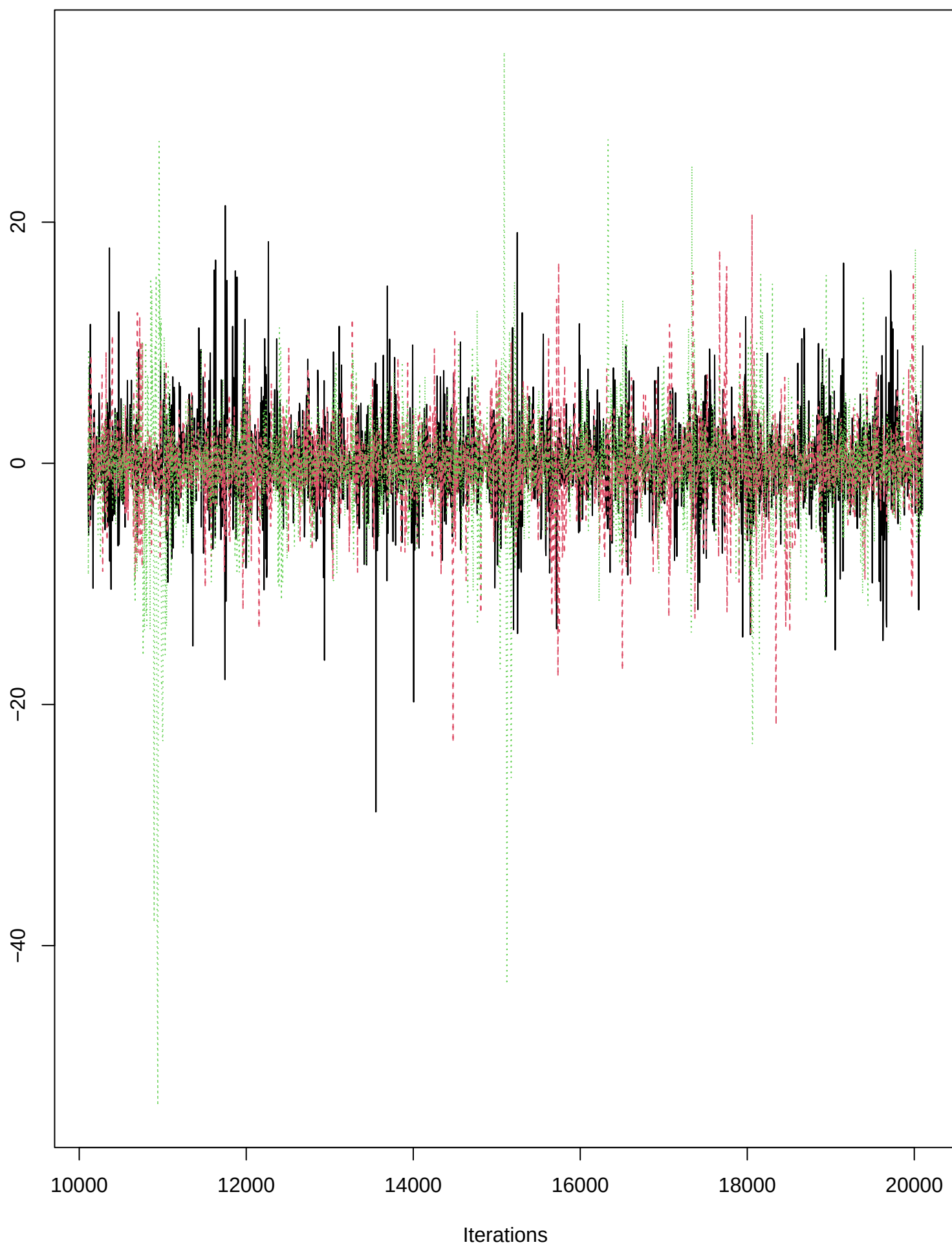
Trace of beta_mon_egg[9]
