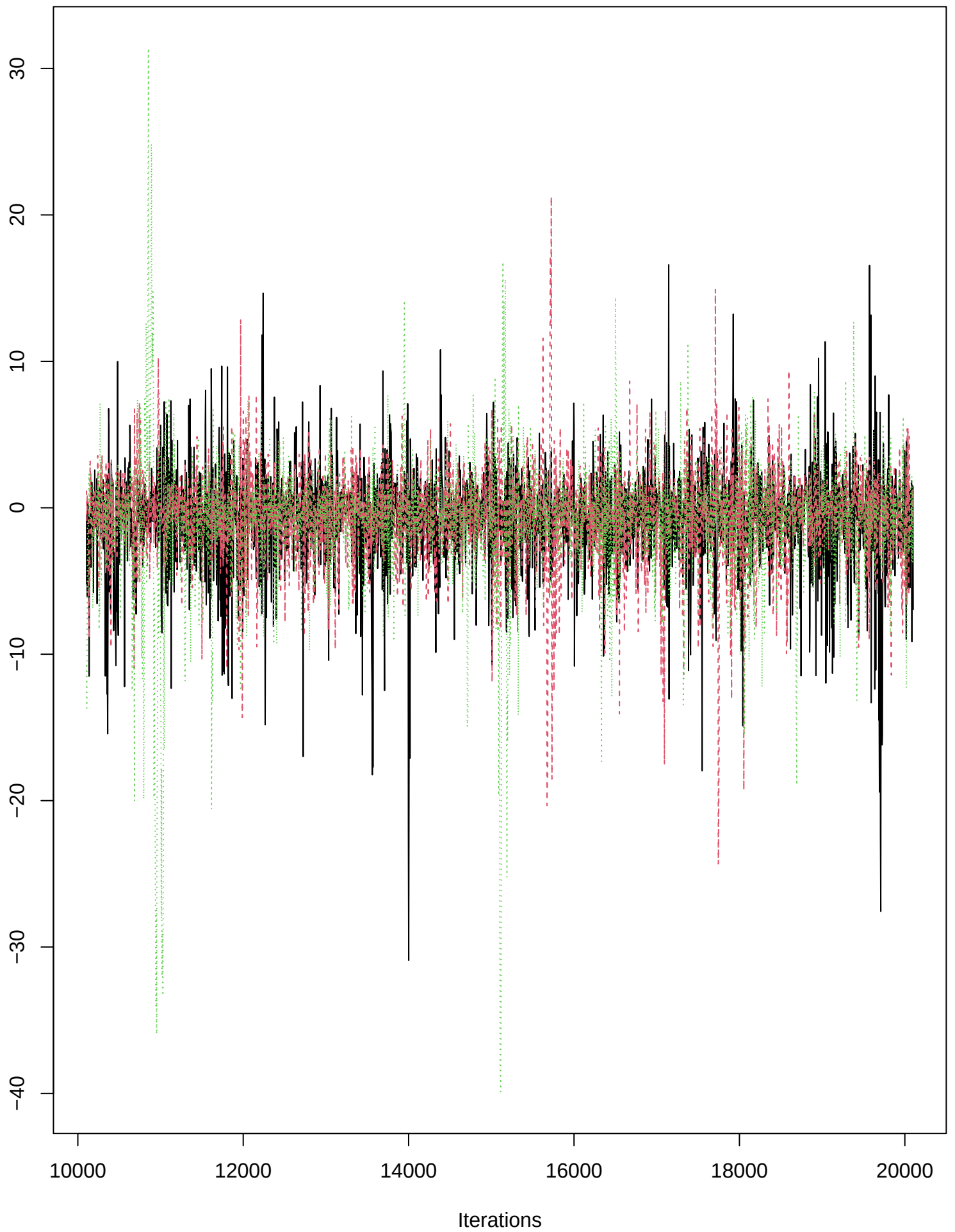
Trace of beta_mon_egg[5]
