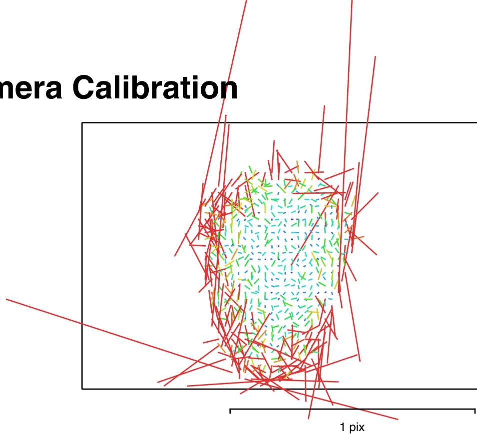
Fig. 3. Image residuals for Canon EOS 2000D, EF-S18-55mm f/3.5-5.6 IS II (24mm).
