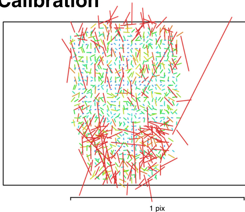
Fig. 2. Image residuals for Canon EOS 2000D,EF-S18-55mm f/3.5-5.6 IS II (29mm).
