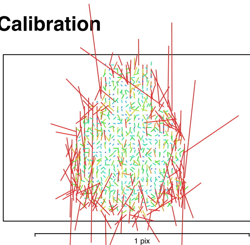
Fig. 3. Image residuals for Canon EOS 2000D, EF-S18-55mm f/3.5-5.6 IS II (24mm).
