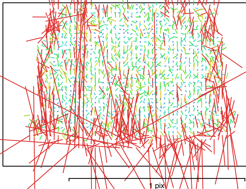
Fig. 2. Image residuals for Canon EOS 2000D, EF-S18-55mm f/3.5-5.6 IS II (20mm).
