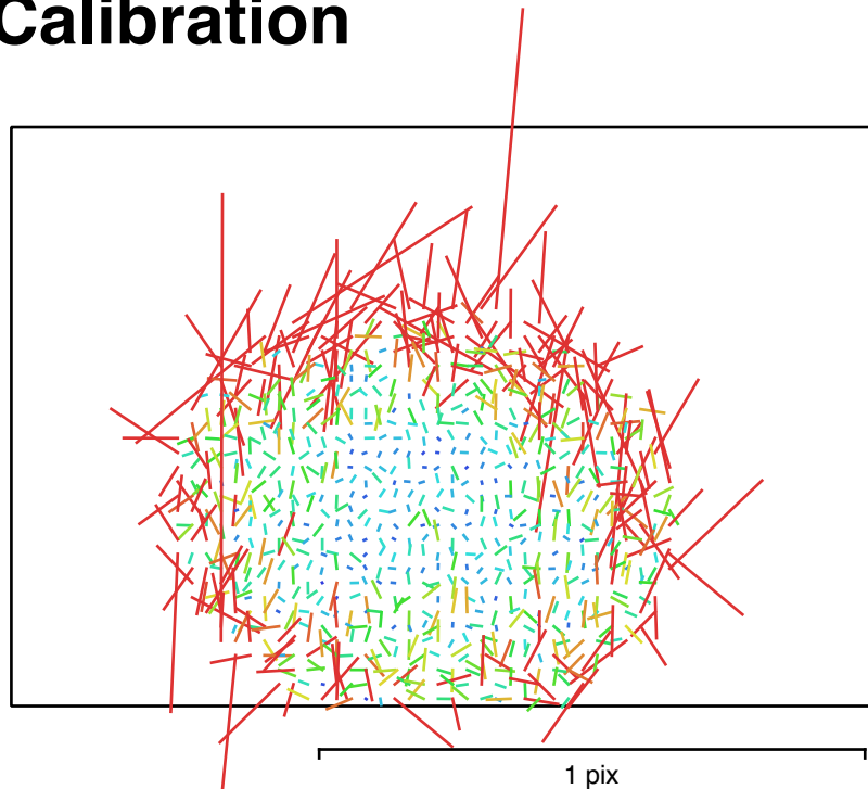
Fig. 4. Image residuals for Canon EOS 2000D, EF-S18-55mm f/3.5-5.6 IS II (35mm).
