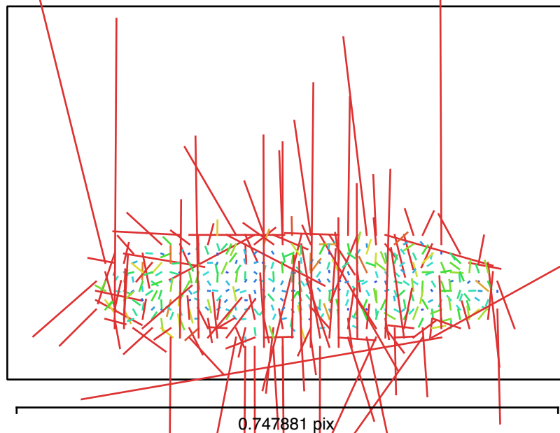
Fig. 2. Image residuals for Canon EOS 2000D, EF-S18-55mm f/3.5-5.6 IS II (28mm).
