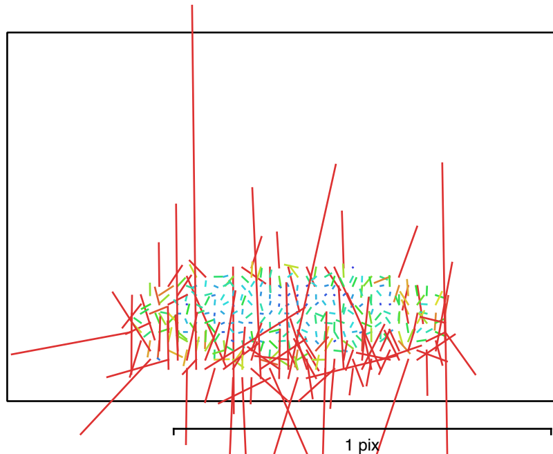
Fig. 3. Image residuals for Canon EOS 2000D, EF-S18-55mm f/3.5-5.6 IS II (41mm).
