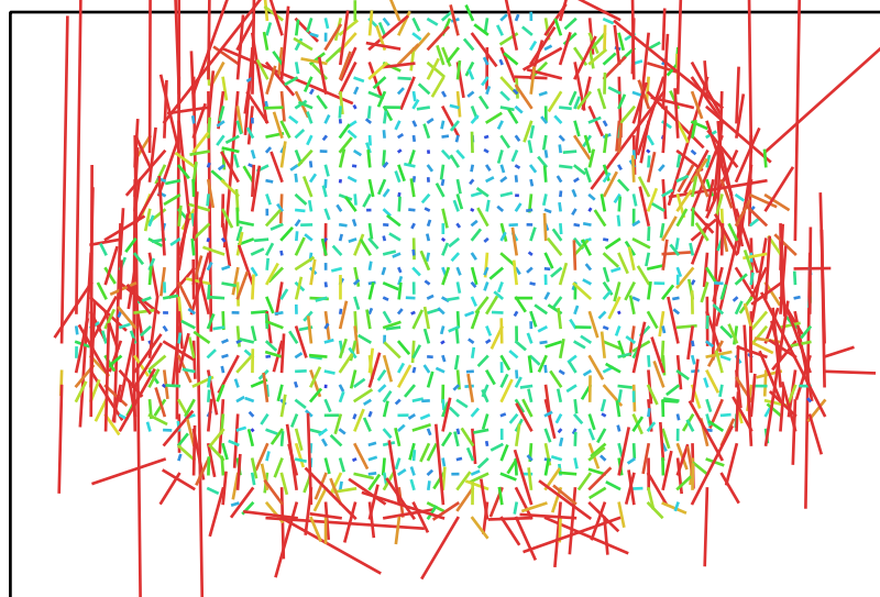
Fig. 3. Image residuals for Canon EOS 2000D, EF-S18-55mm f/3.5-5.6 IS II (27mm).
