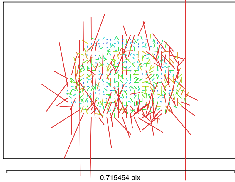
Fig. 2. Image residuals for Canon EOS 2000D, EF-S18-55mm f/3.5-5.6 IS II (30mm).
