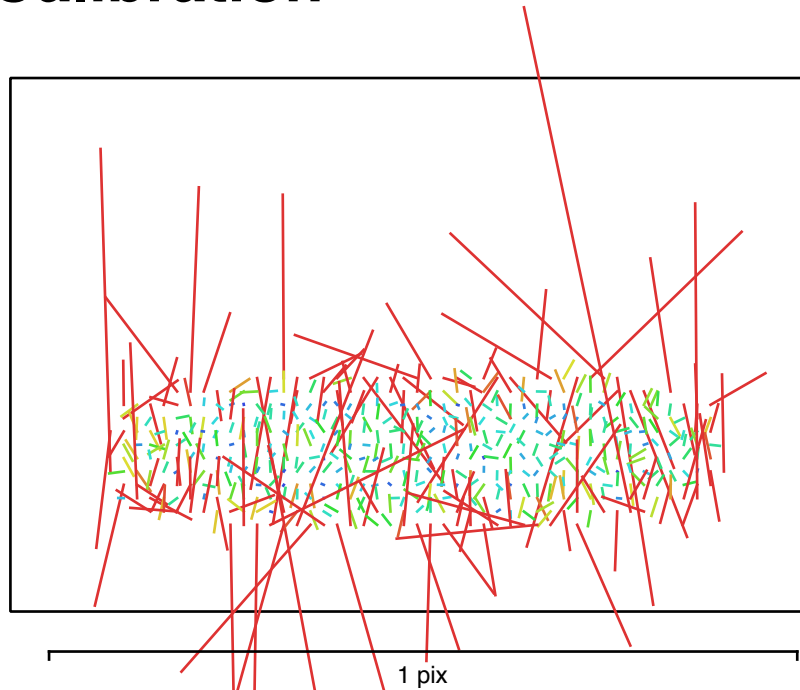
Fig. 3. Image residuals for Canon EOS 2000D, EF-S18-55mm f/3.5-5.6 IS II (42mm).
