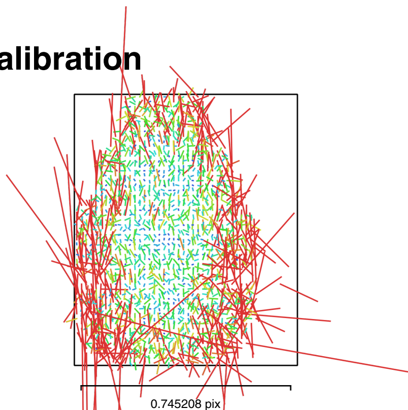
Fig. 4. Image residuals for EOS 2000D, Canon EF-S 18-55mm f/3.5-5.6 IS II (27mm).
