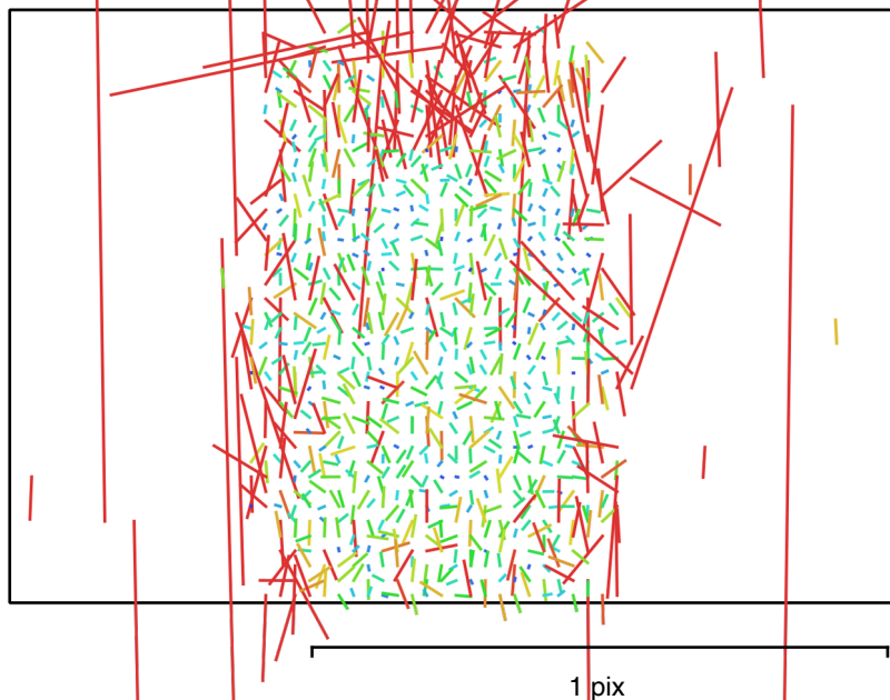
Fig. 2. Image residuals for EOS 2000D, Canon EF-S18-55mm f/3.5-5.6 IS II (41mm).
