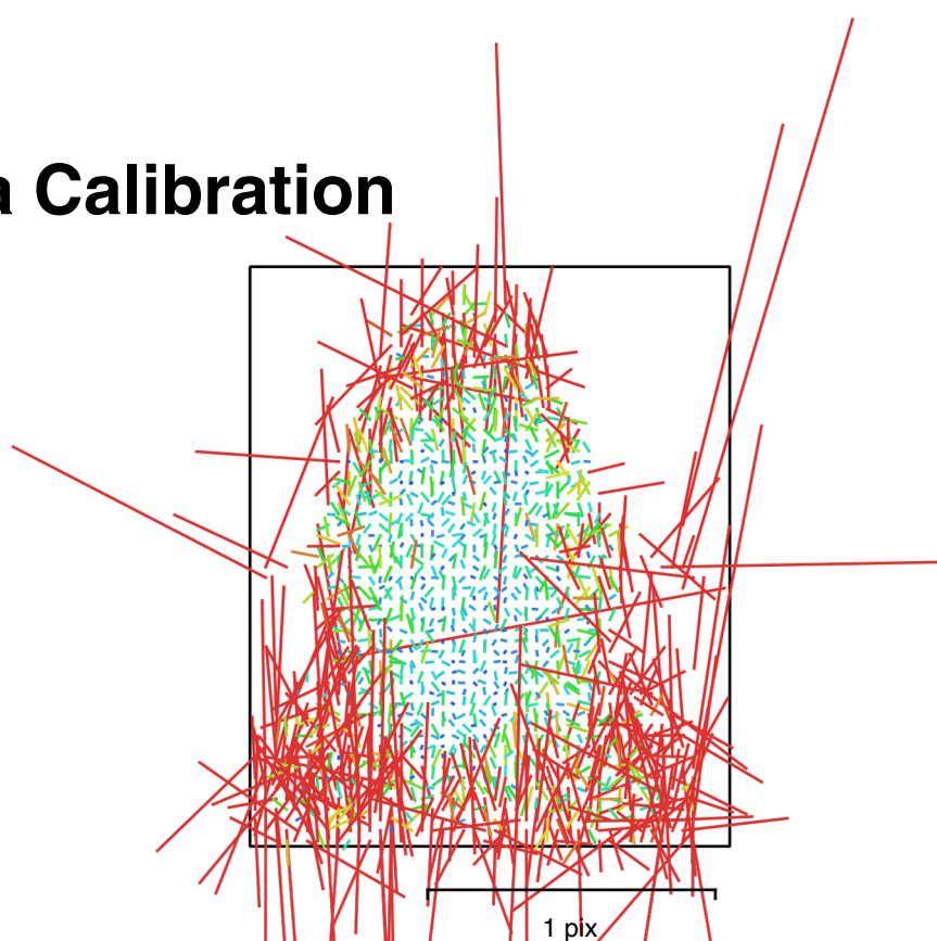
Fig. 3. Image residuals for EOS 2000D, Canon EF-S 18-55mm f/3.5-5.6 IS II (27mm).
