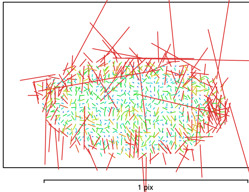
Fig. 2. Image residuals for Canon EOS 2000D, EF-S18-55mm f/3.5-5.6 IS II (32mm).
