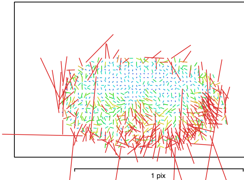
Fig. 3. Image residuals for Canon EOS 2000D, EF-S18-55mm f/3.5-5.6 IS II (25mm).
