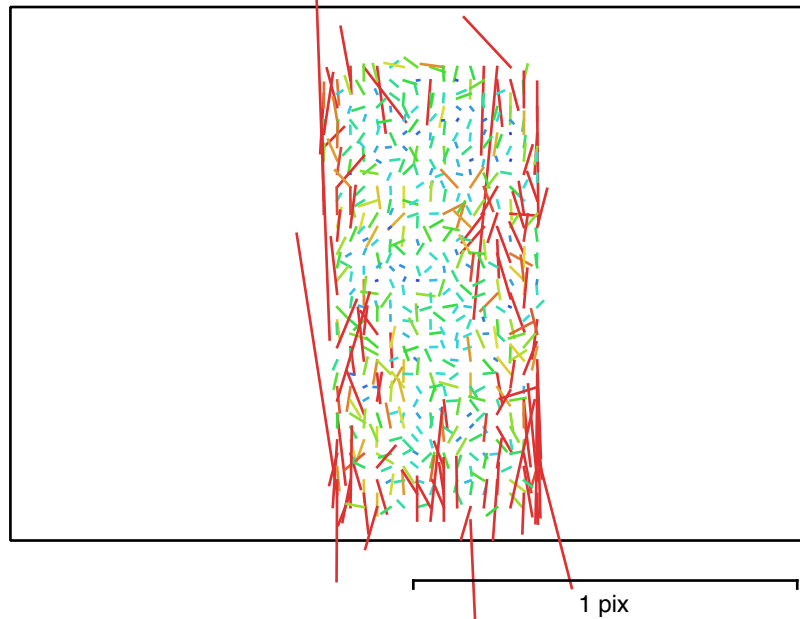
Fig. 2. Image residuals for Canon EOS 2000D, EF-S18-55mm f/3.5-5.6 IS II (25mm).
