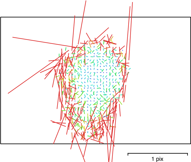
Fig. 3. Image residuals for Canon EOS 2000D, EF-S18-55mm f/3.5-5.6 IS II (24mm).
