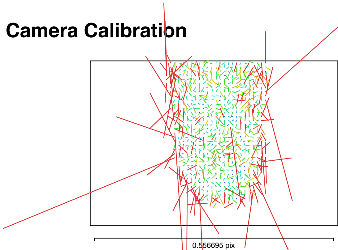
Fig. 2. Image residuals for Canon EOS 2000D, EF-S18-55mm f/3.5-5.6 IS II (21mm).
