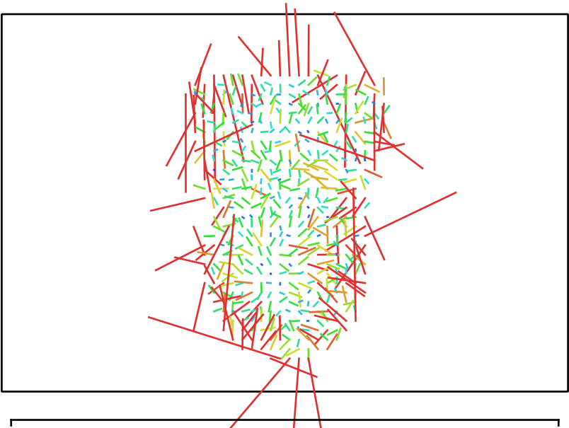
Fig. 3. Image residuals for Canon EOS 2000D, EF-S18-55mm f/3.5-5.6 IS II (32mm).
