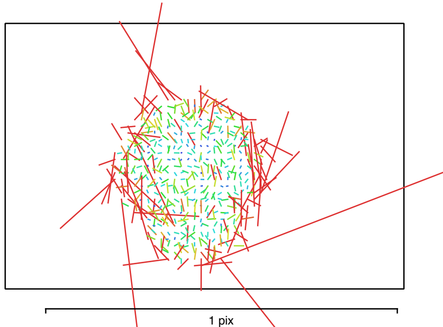
Fig. 4. Image residuals for Canon EOS 2000D, EF-S18-55mm f/3.5-5.6 IS II (25mm).
