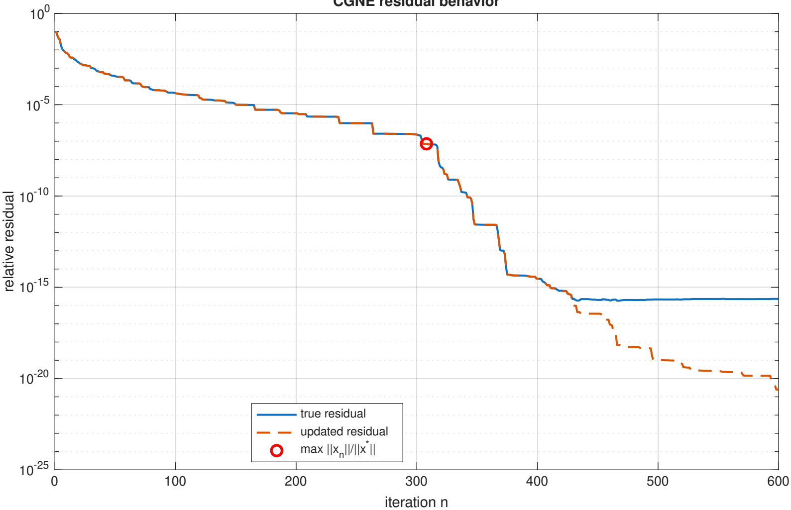
CGNE residual behavior
