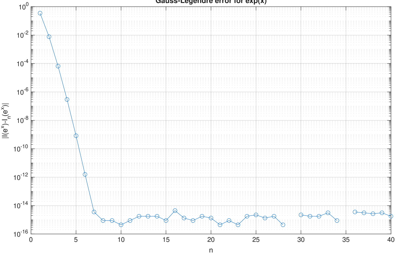
Gauss-Legendre error for \exp(x)
