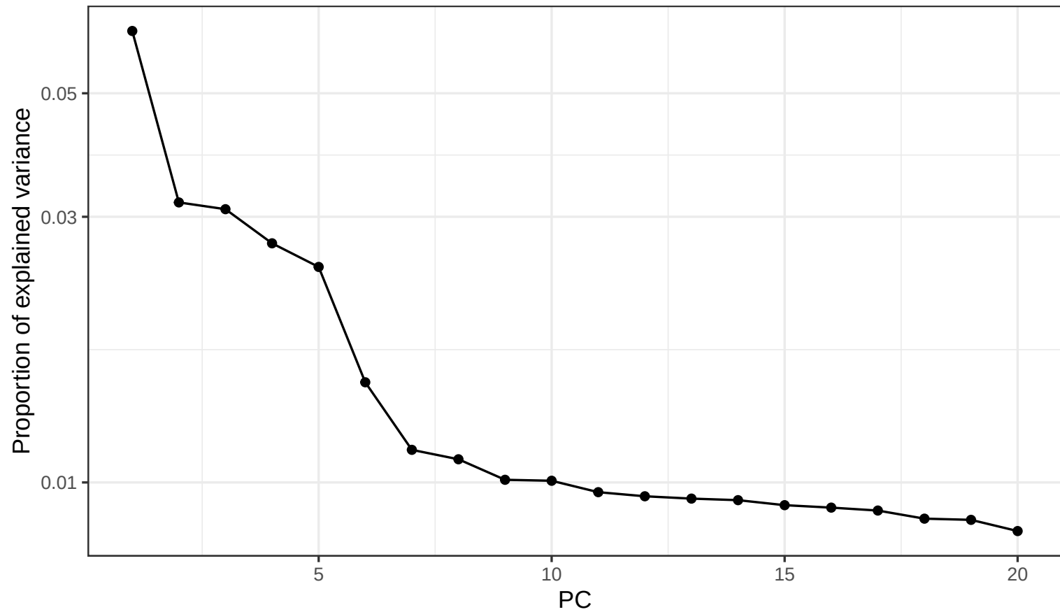
Scree Plot – K = 20
