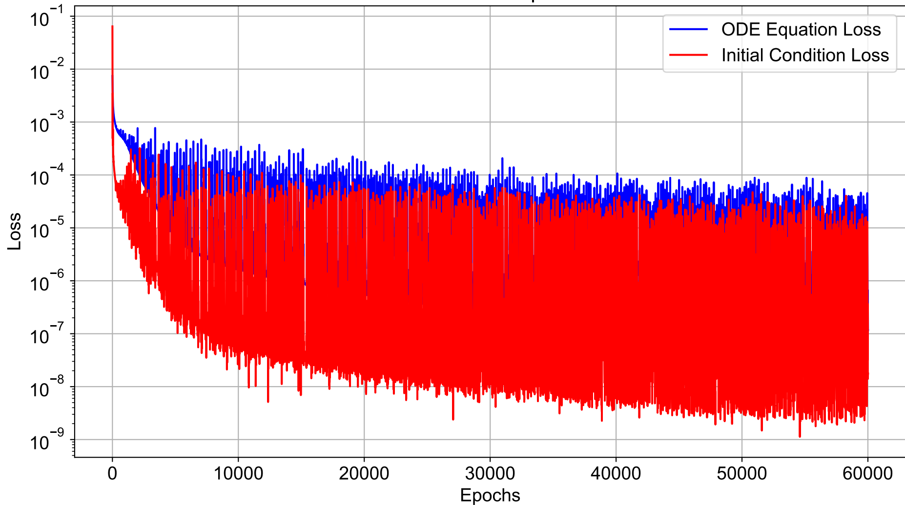
Loss Across Epochs
