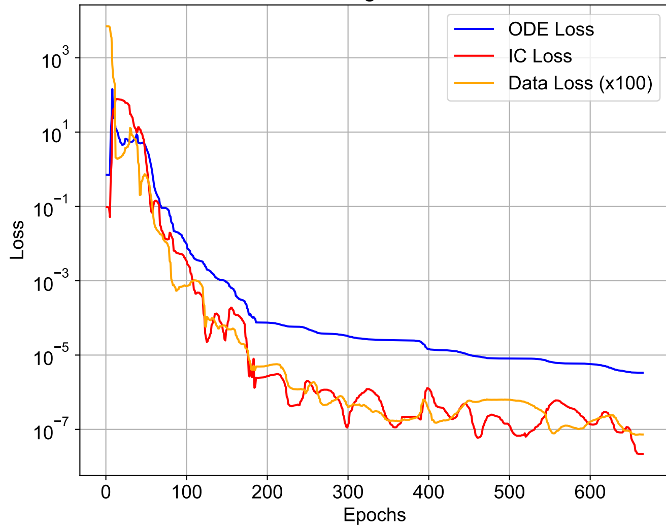
Training Losses
