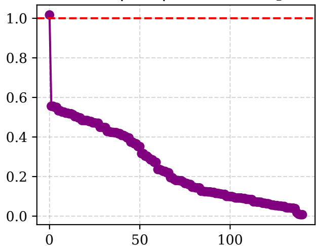
ecDAE |\lambda(A)| for walk slope
