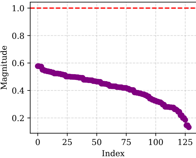
cDAE |\lambda(A)| for push door
