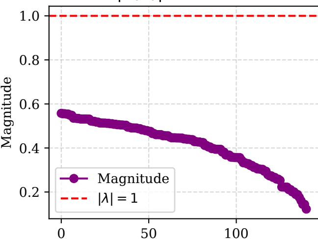
cDAE |\lambda(A)| for stand dance
