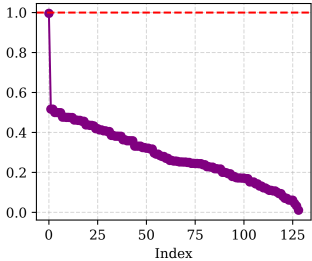
ecDAE |\lambda(A)| for push door
