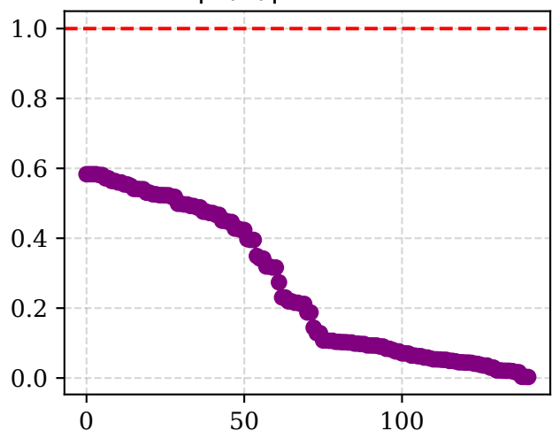
ecDAE |\lambda(A)| for stand dance
