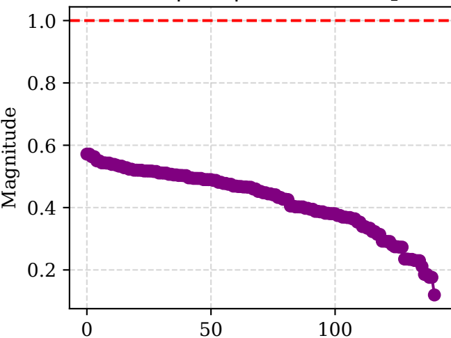
cDAE |\lambda(A)| for walk slope
