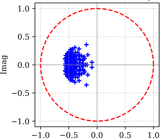
cDAE \lambda(A) for push door
