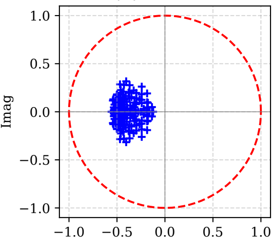
cDAE \lambda(A) for walk slope
