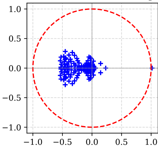
ecDAE \lambda(A) for push door
