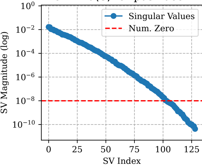
cDAE \sigma(C) for push door
