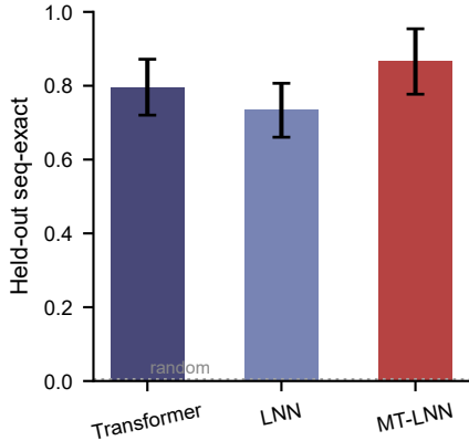
Selective Copy (T=37, 1500 steps)
