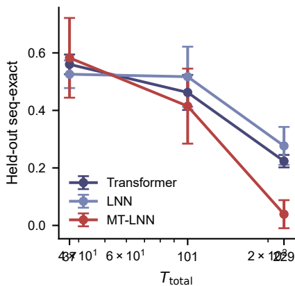
Long-context sweep (600/500 steps)
