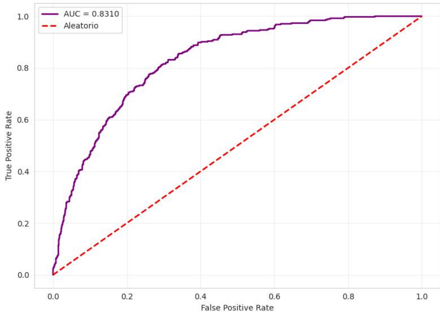
Curva ROC — Red Neuronal
