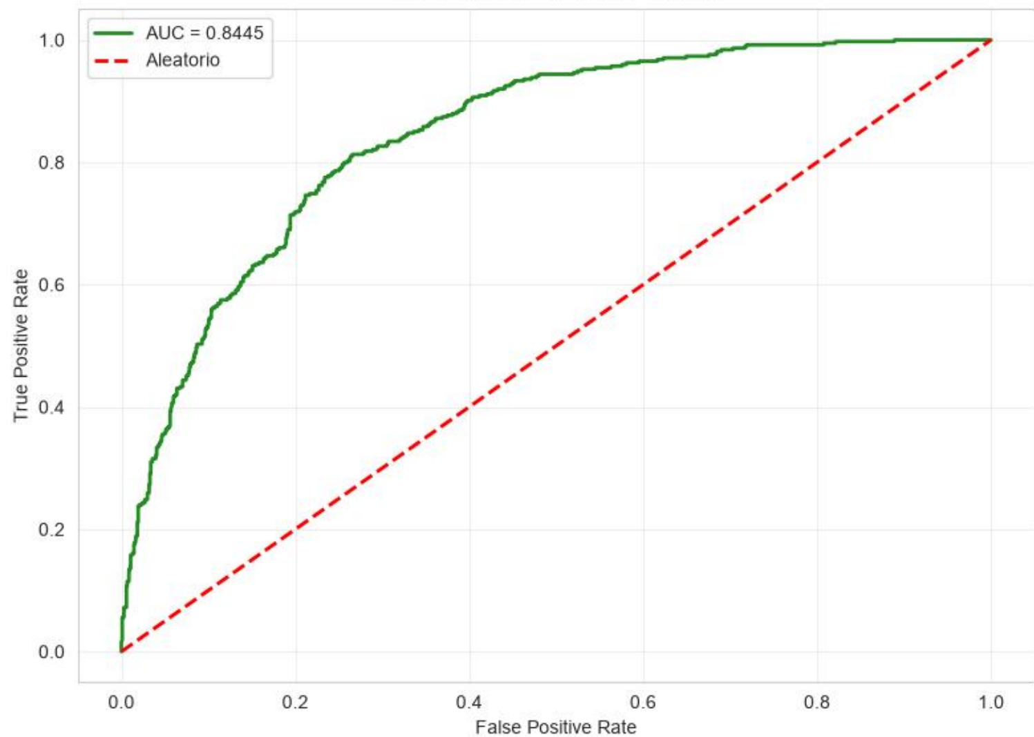
Curva ROC — Random Forest
