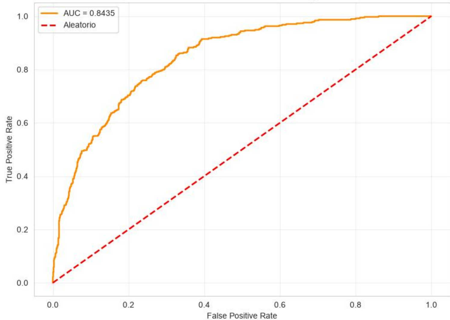
Curva ROC — Gradient Boosting
