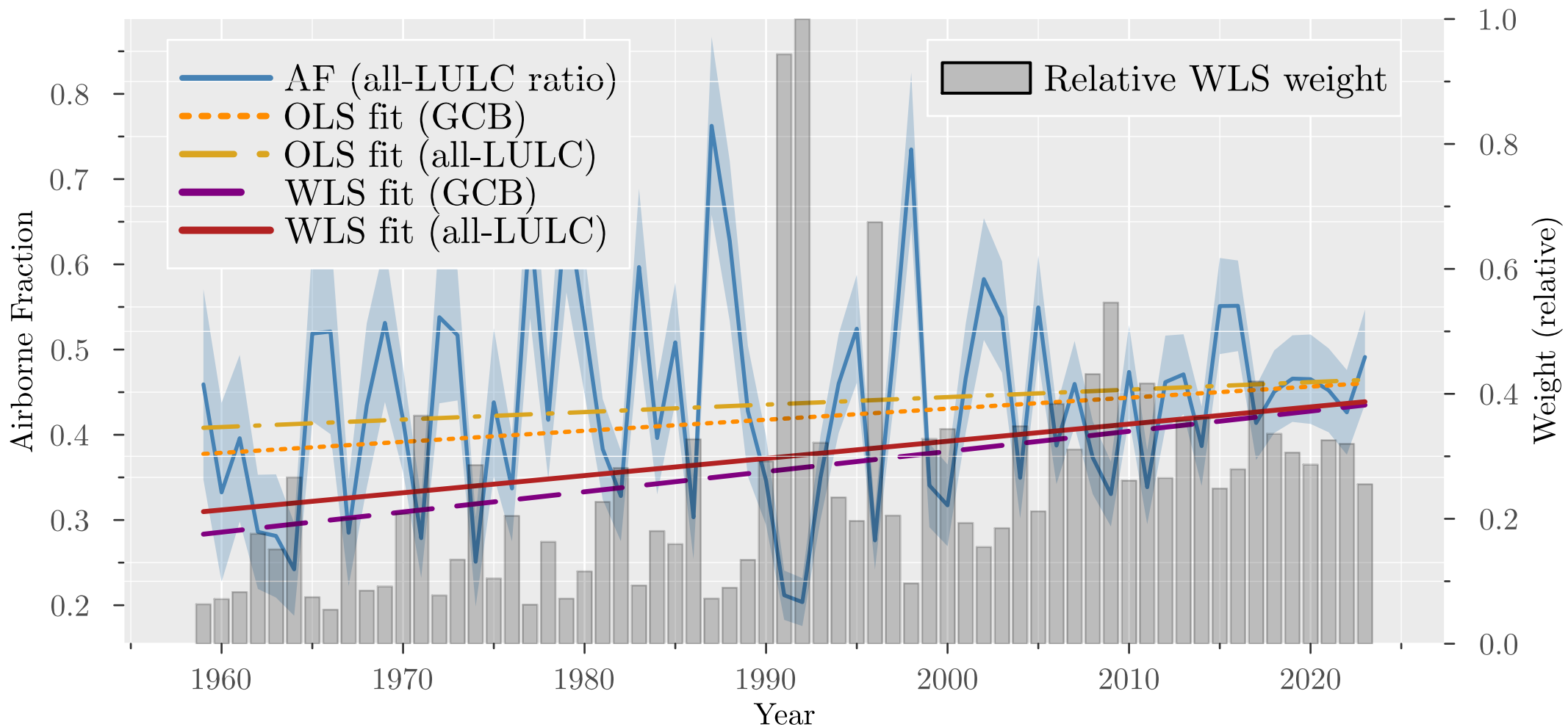
Airborne Fraction with OLS and WLS fits for all LULC measurements, without 2024
