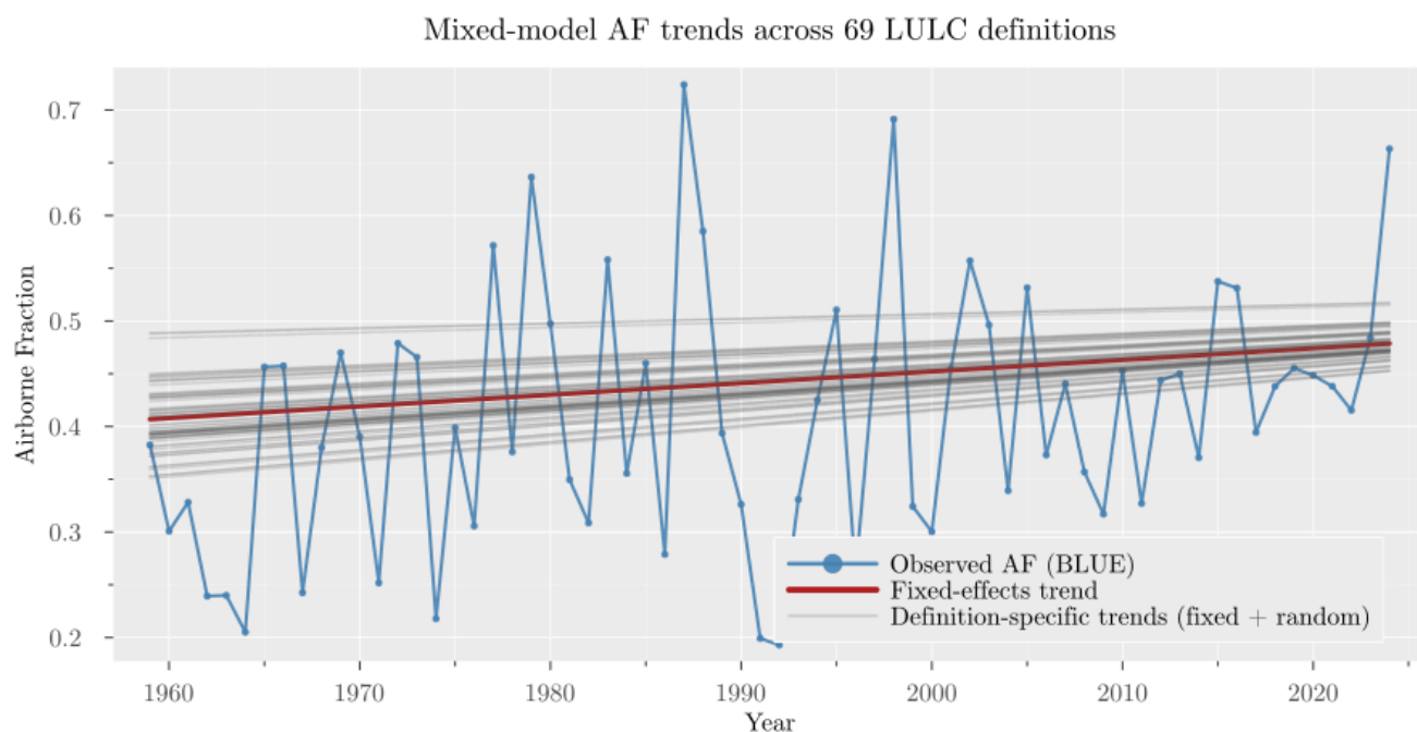
85 86 (a) AF series with mixed-effects model trend (full sample, 1959-2024).
