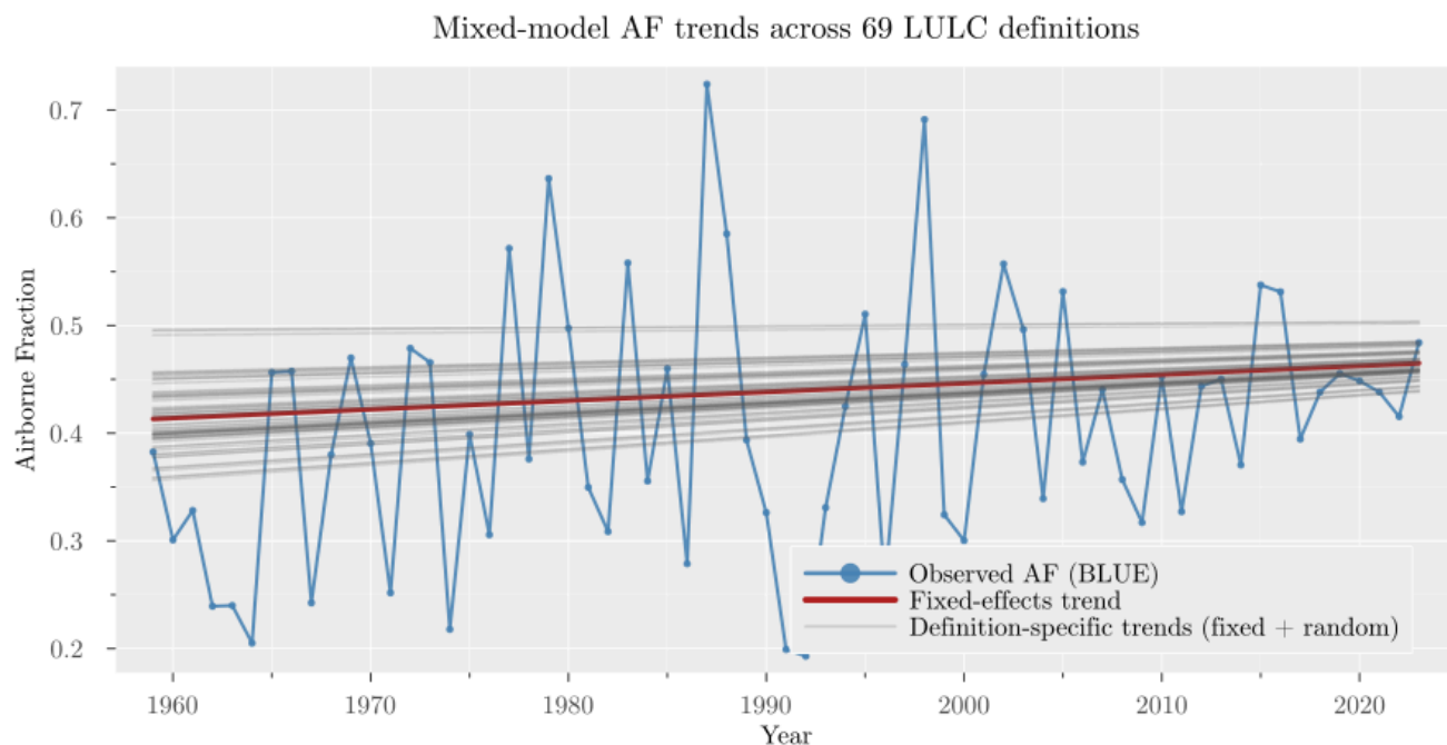
87 88 (b) AF series with mixed-effects model trend (sample ending in 2023).
