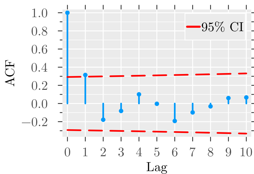
Autocorrelation function
