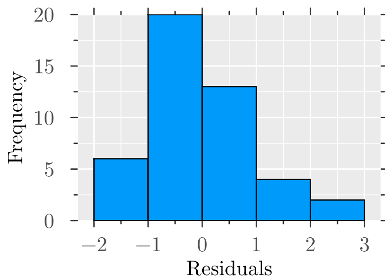
Histogram
