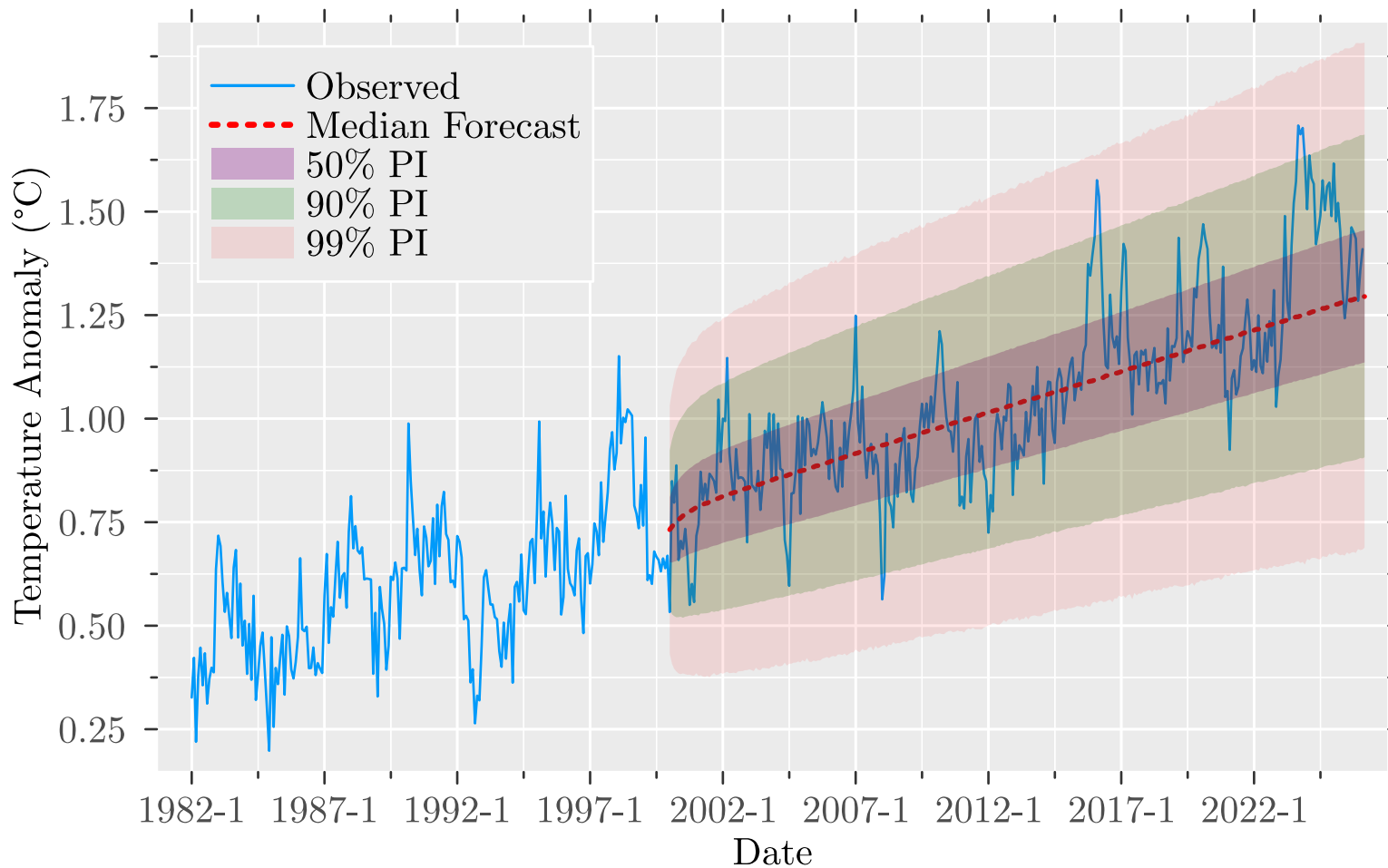
Forecasted Temperature with PI (HadCRUT)
